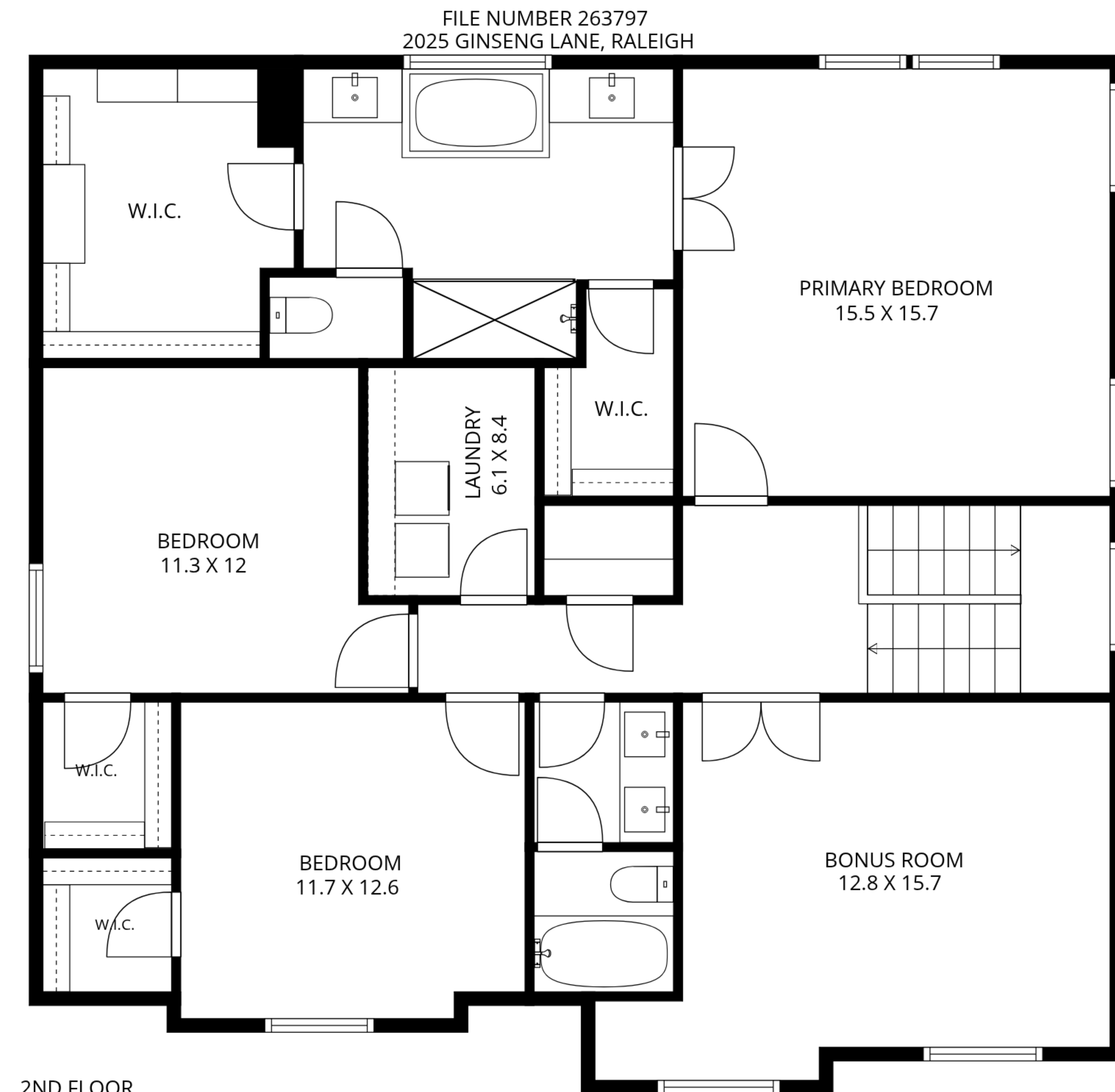
2ND FLOOR
