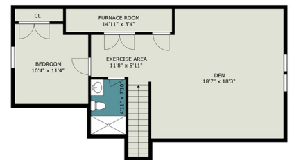
Third Floor
