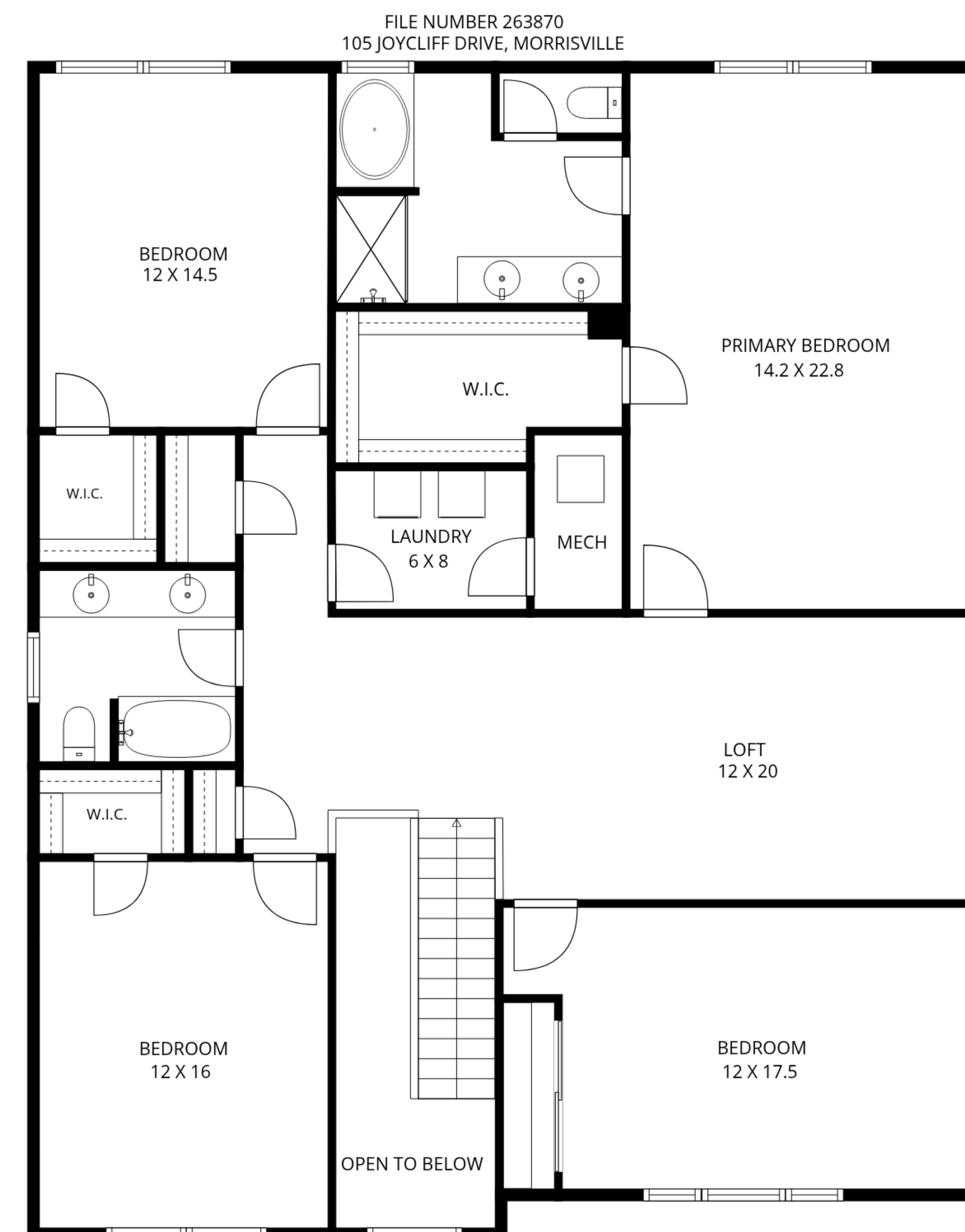
2ND FLOOR
