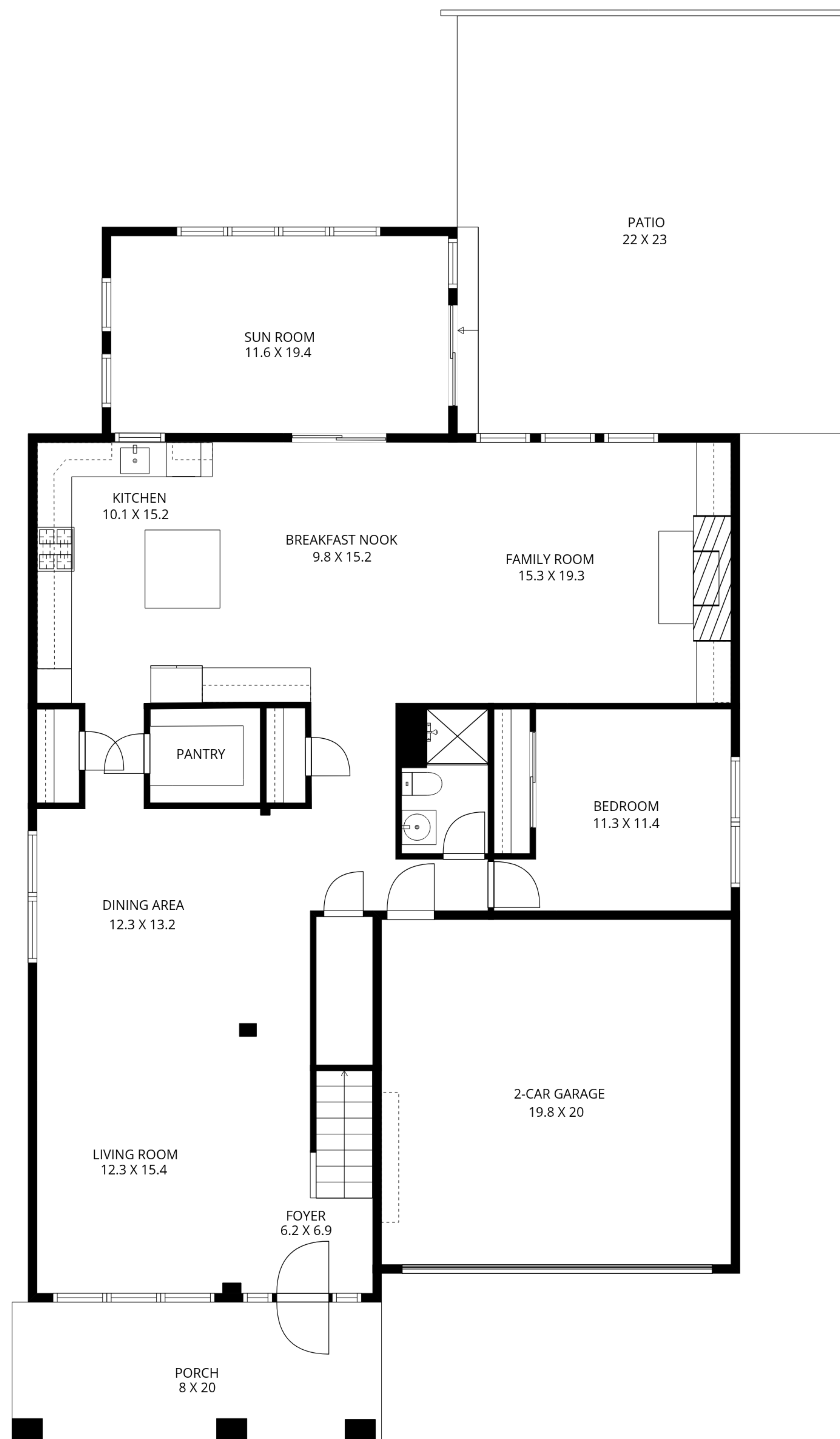
1ST FLOOR
