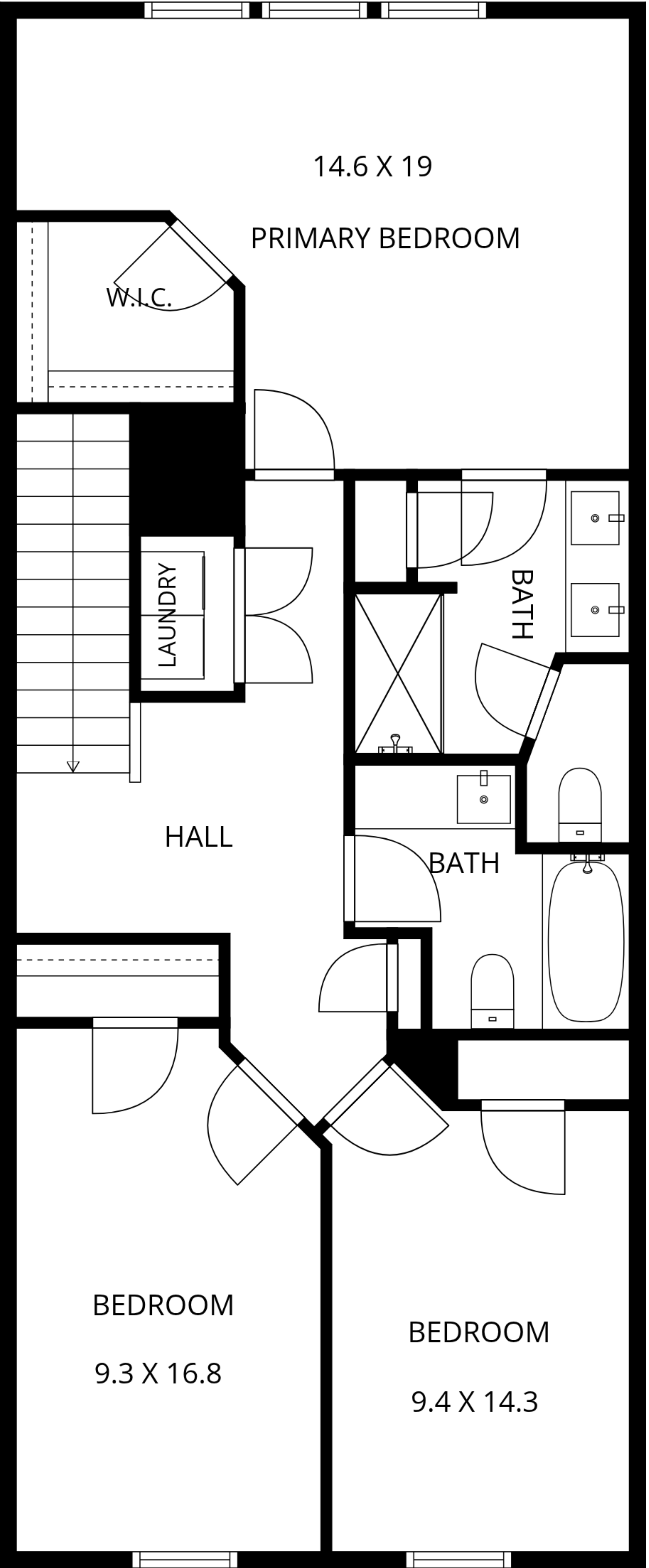
2ND FLOOR
