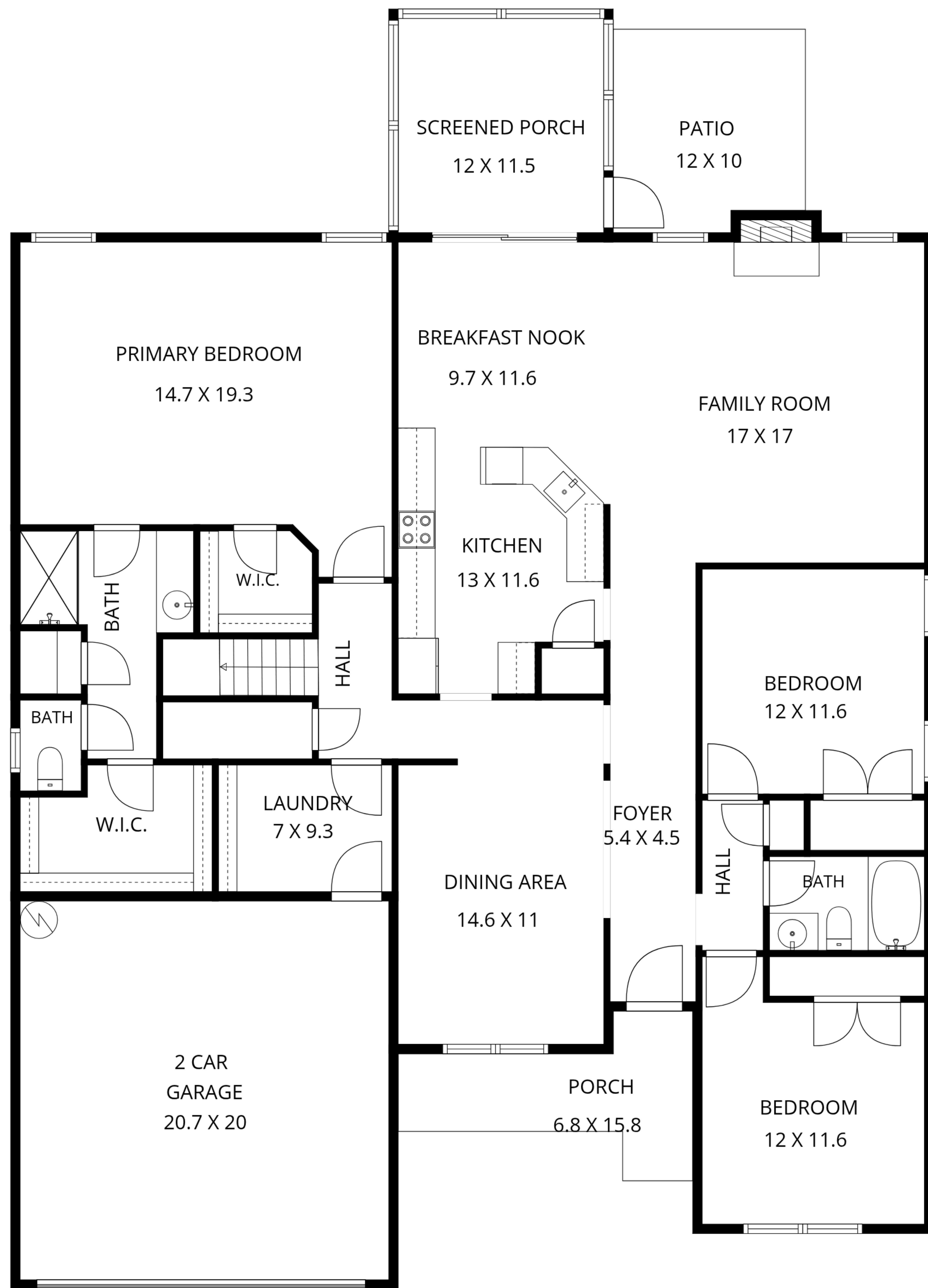
1ST FLOOR
