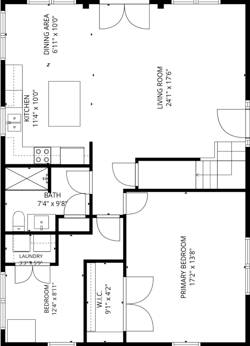
2nd floor
