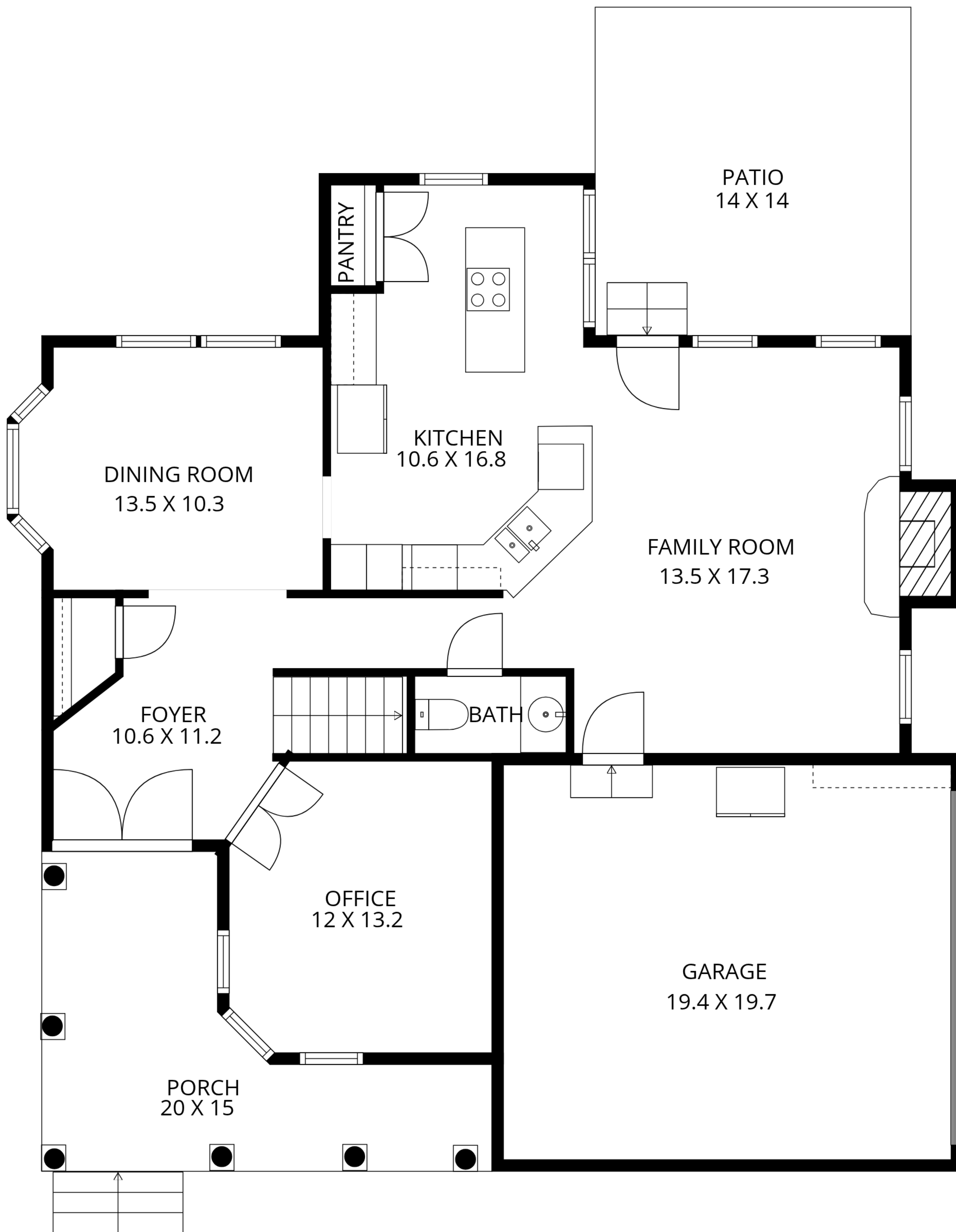
1ST FLOOR
