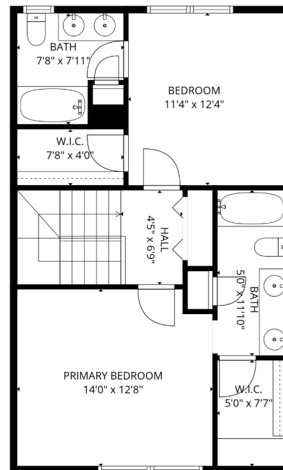
2nd floor
