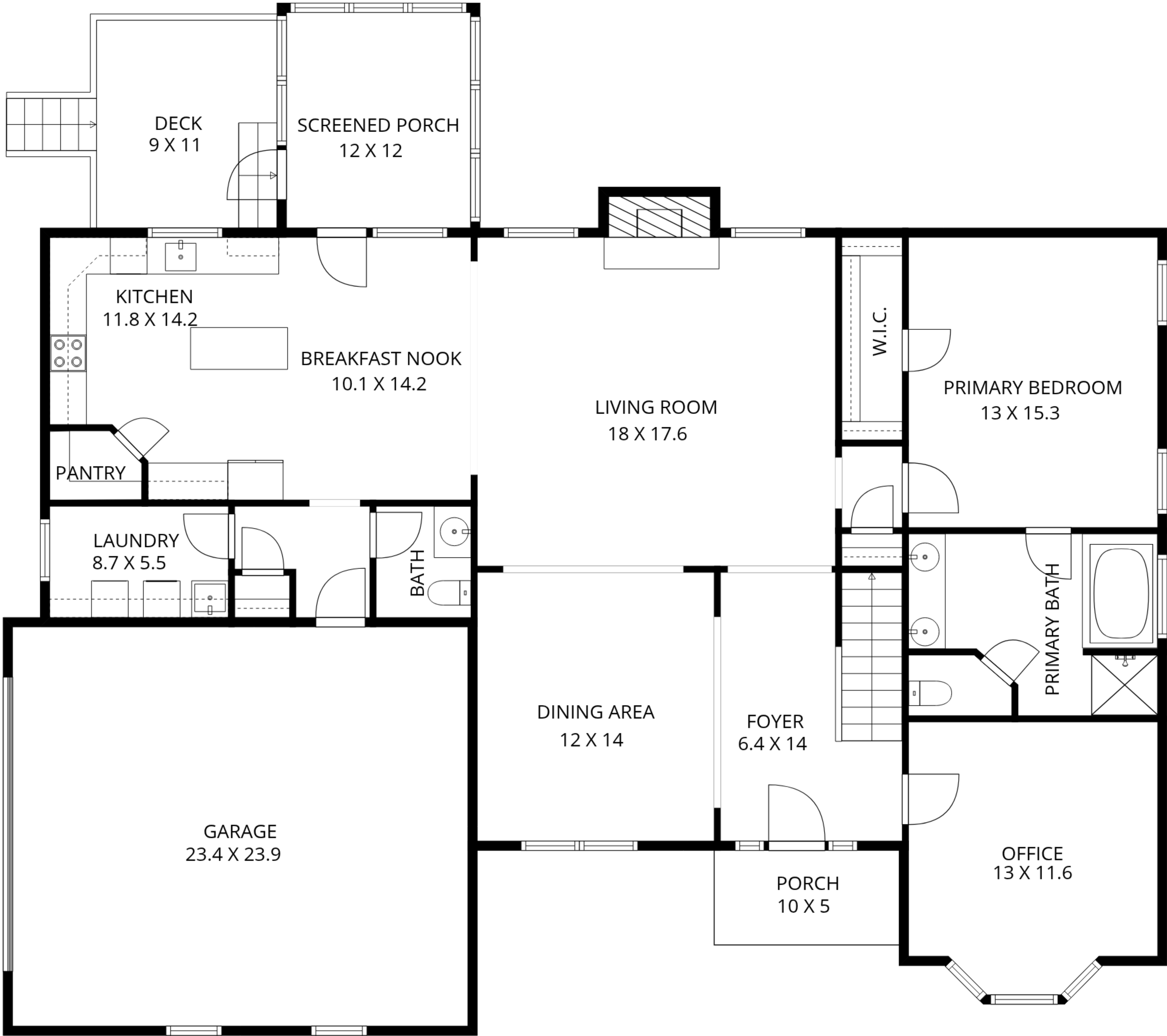
1ST FLOOR
