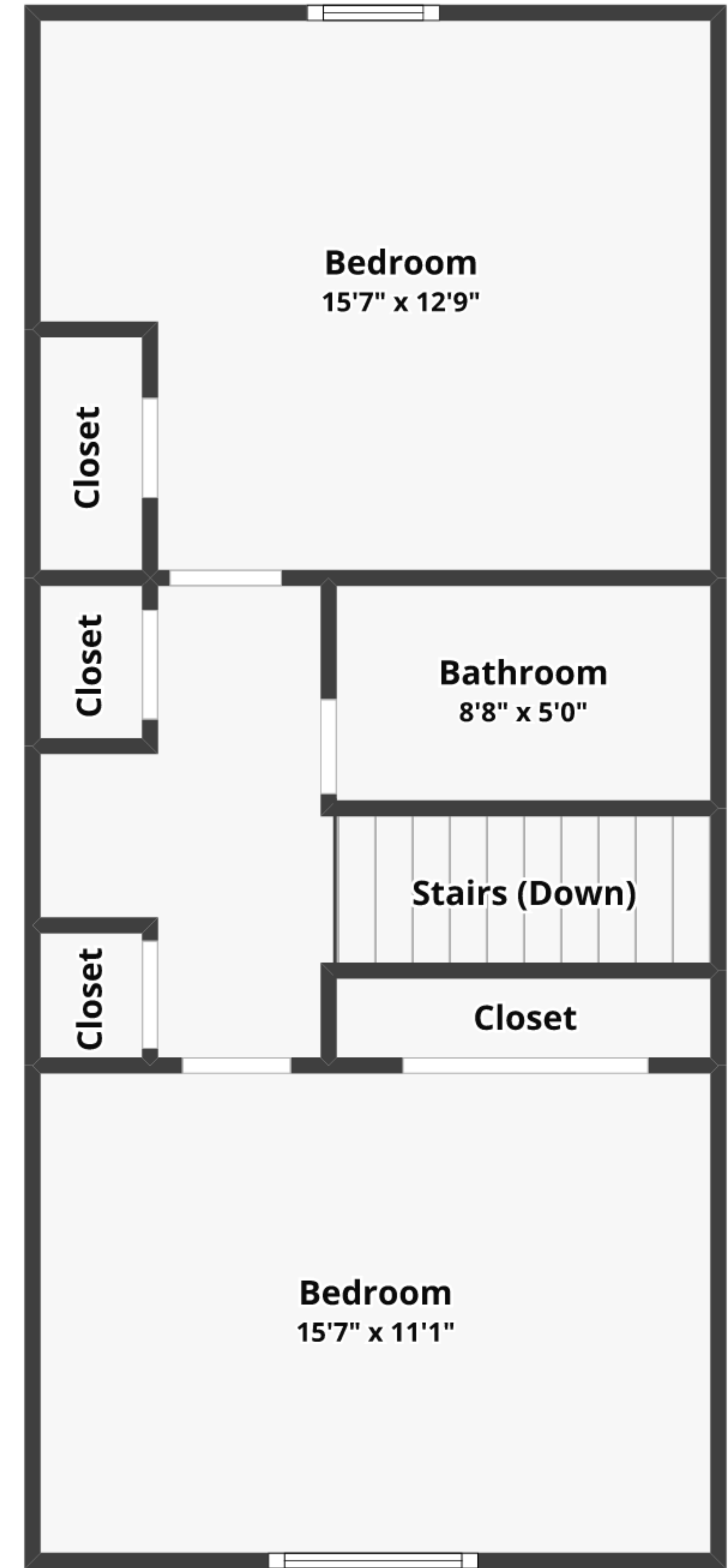
FLOOR 2
