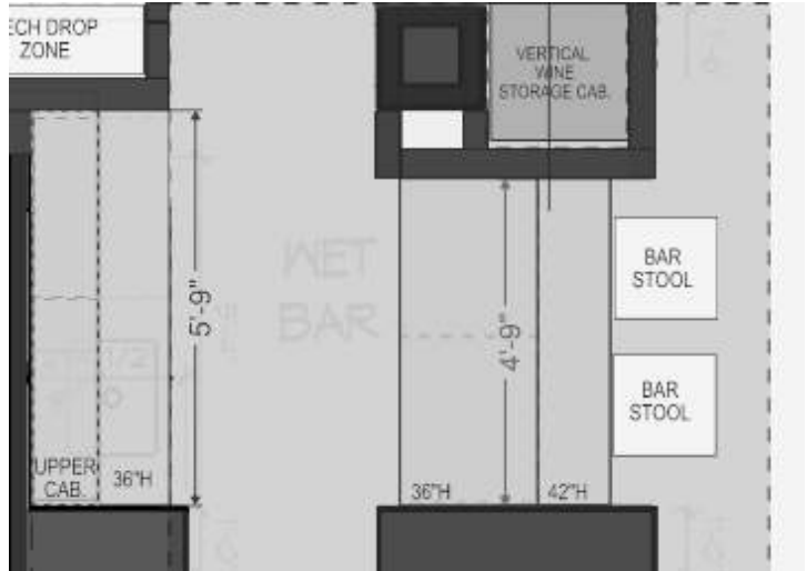
SKETCH FLOOR PLAN, NTS
