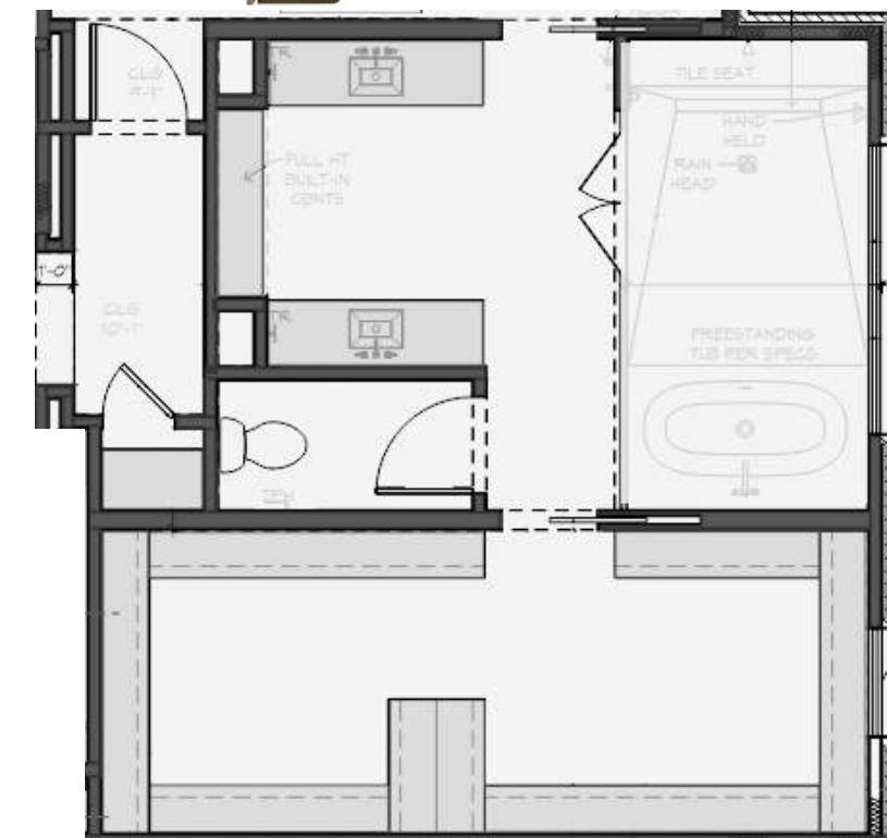
SKETCH FLOOR PLAN, NTS
