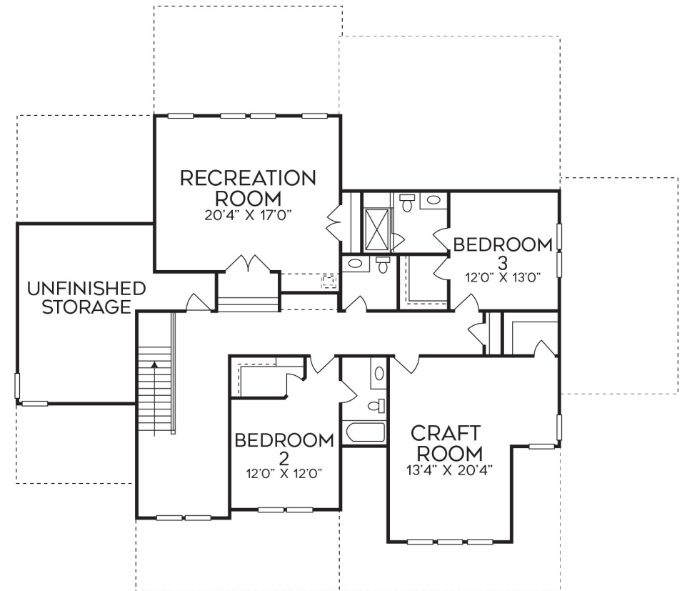
SECOND FLOOR
