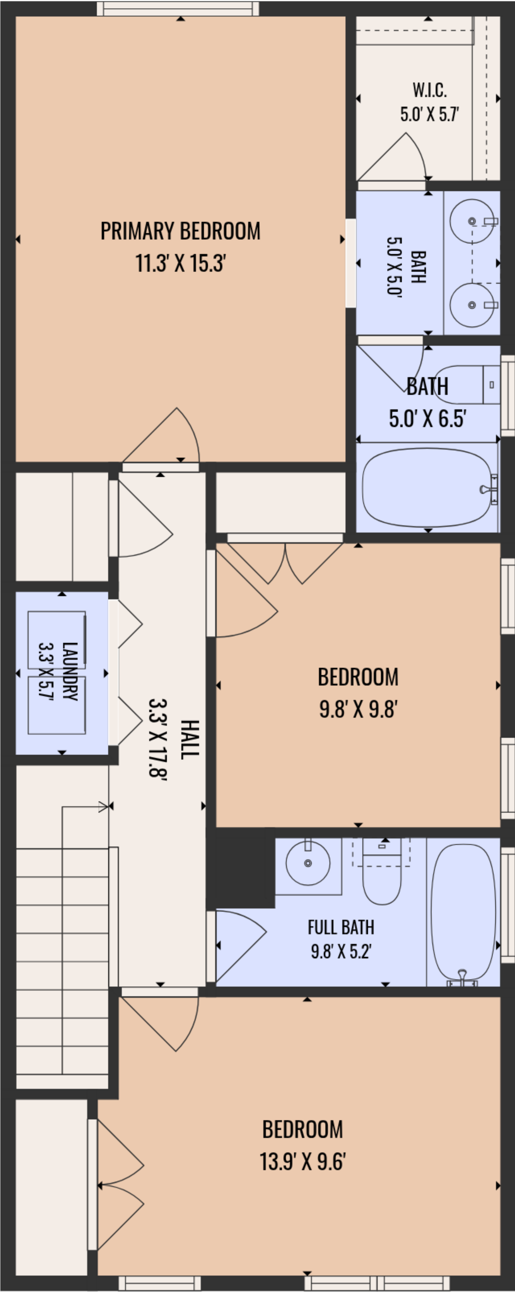
2ND FLOOR
