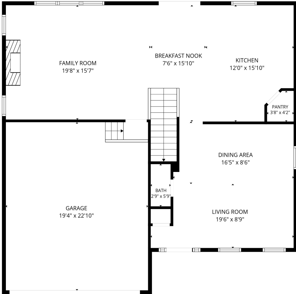
1st floor
