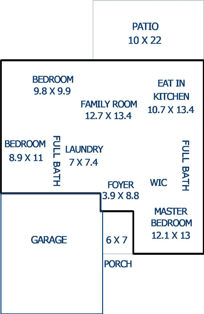
APPROXIMATE DIMENSIONS
