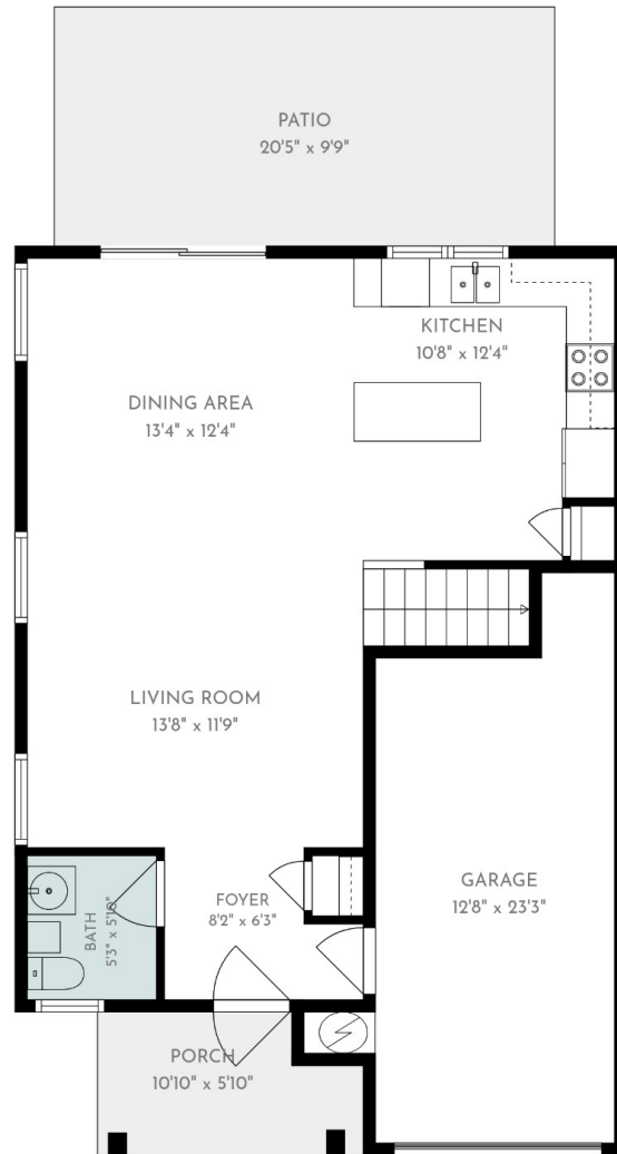
1st floor
