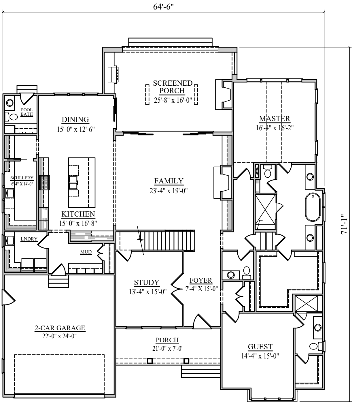
1ST FLOOR
