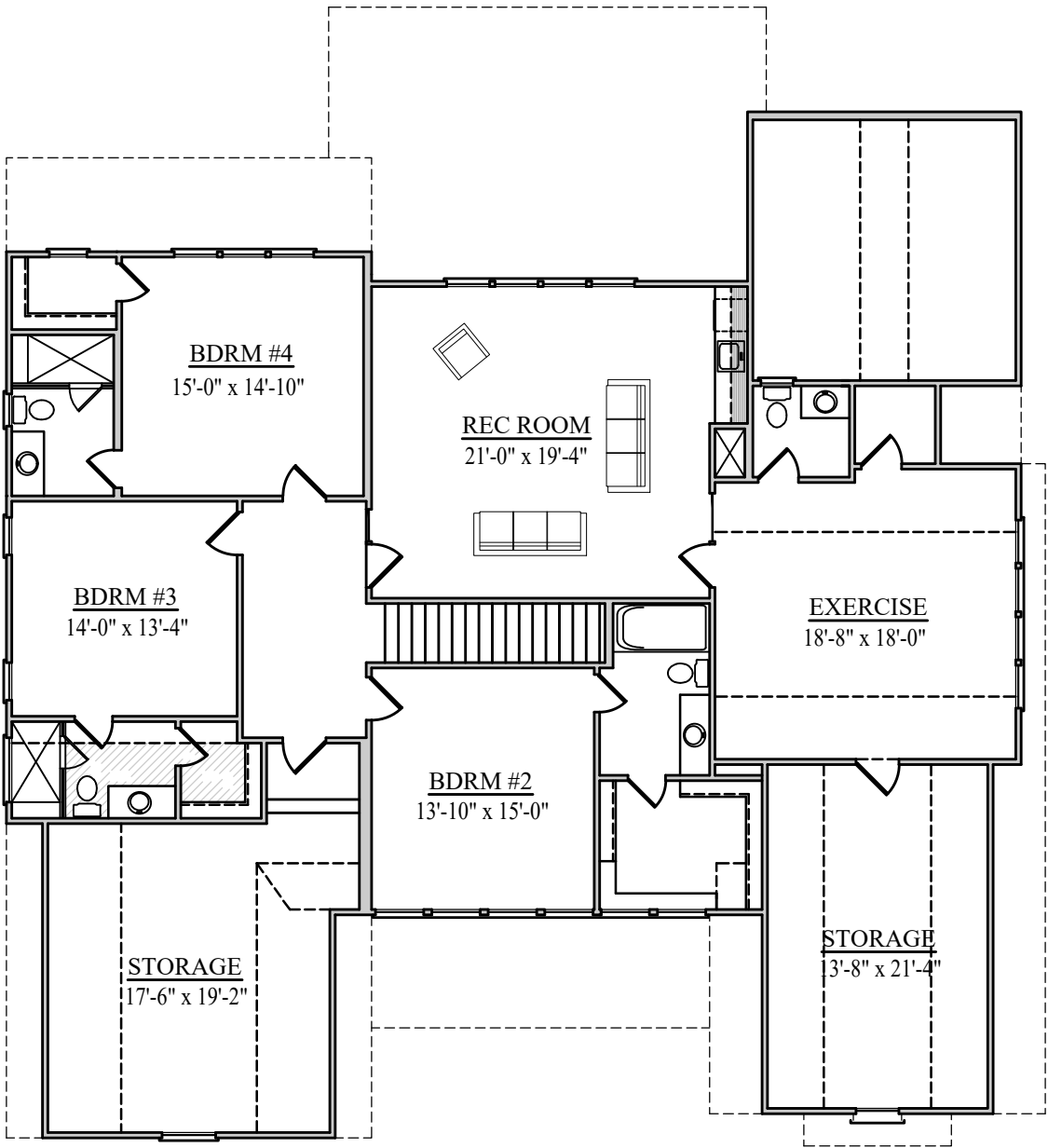
2ND FLOOR
