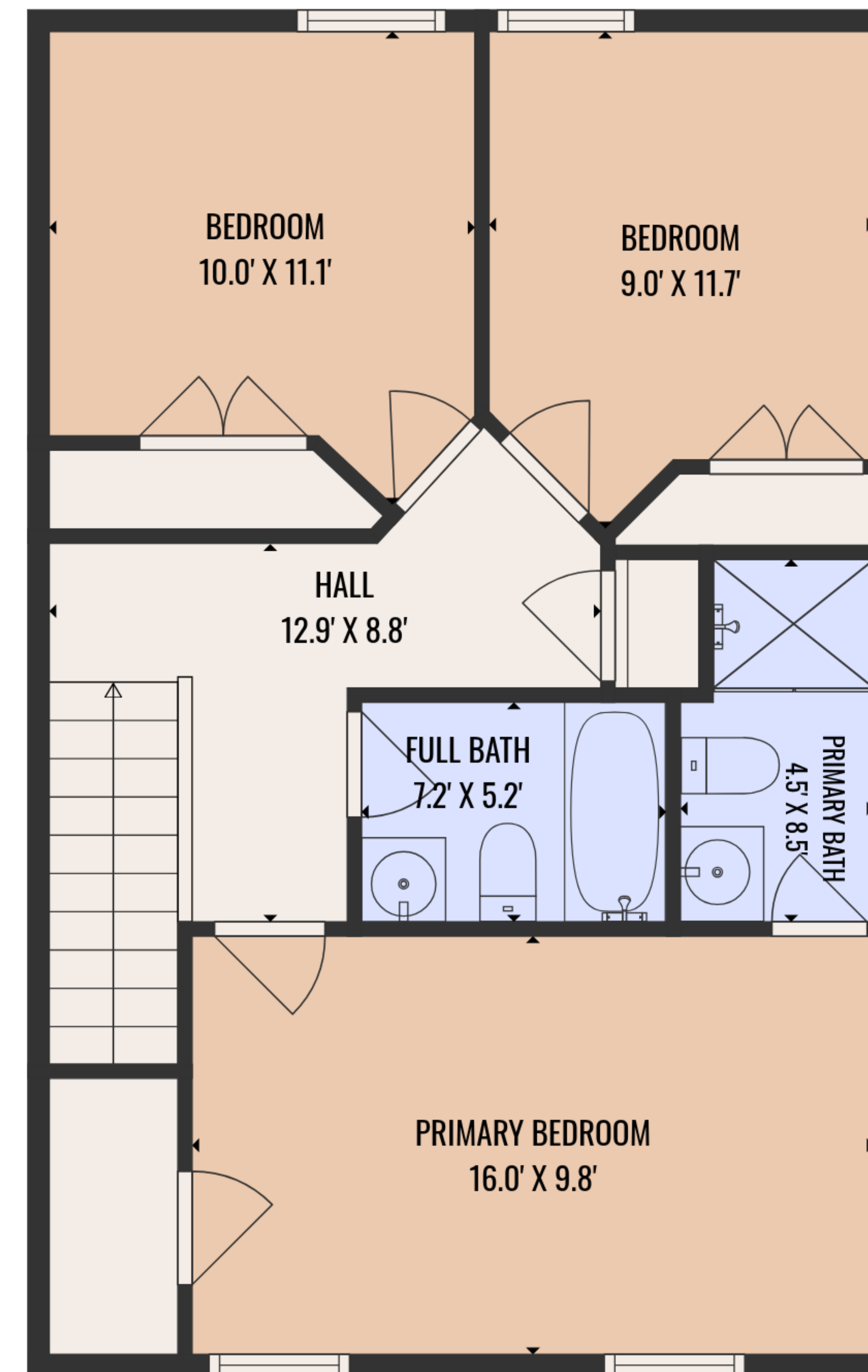
2ND FLOOR
