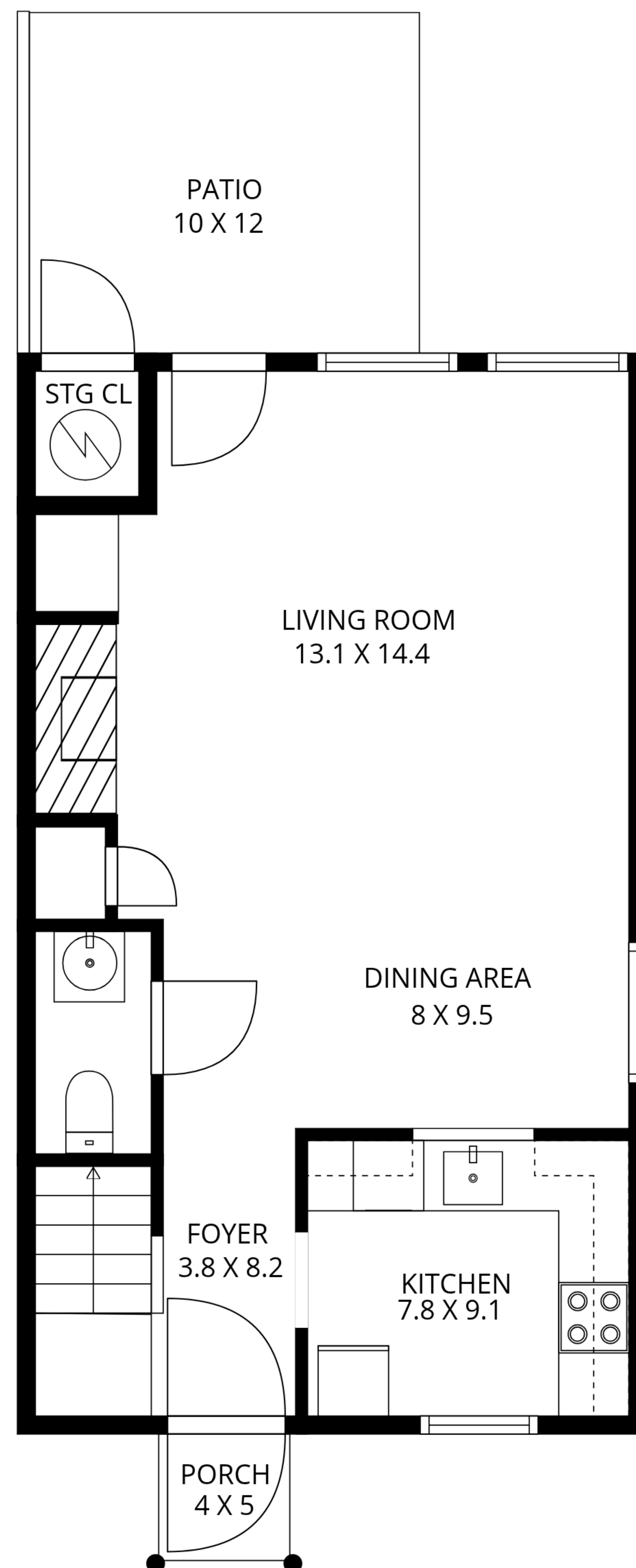
1ST FLOOR
