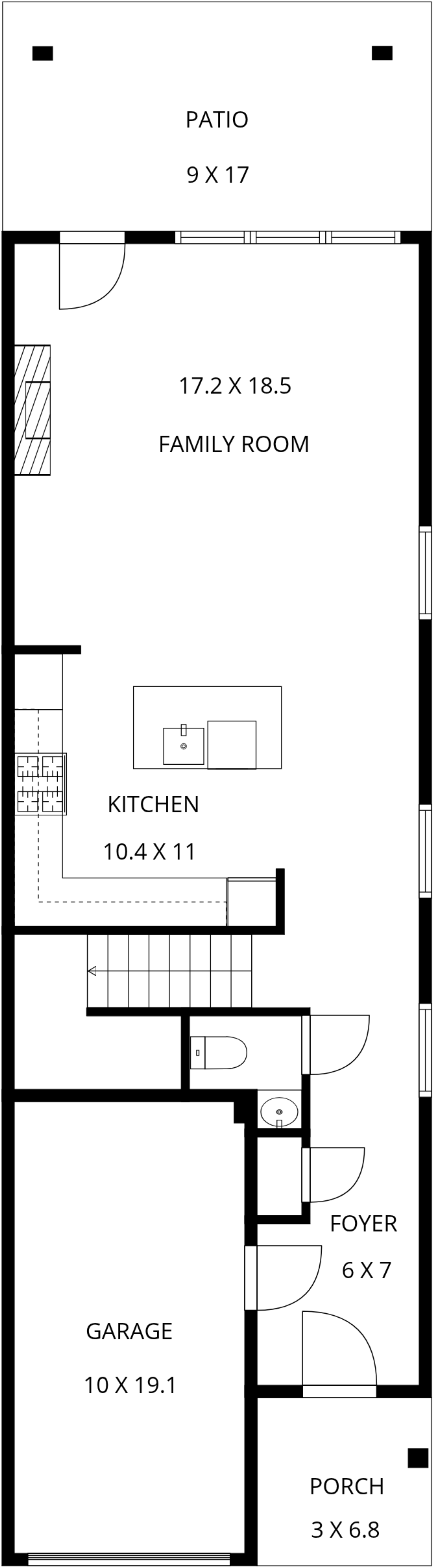
1ST FLOOR
