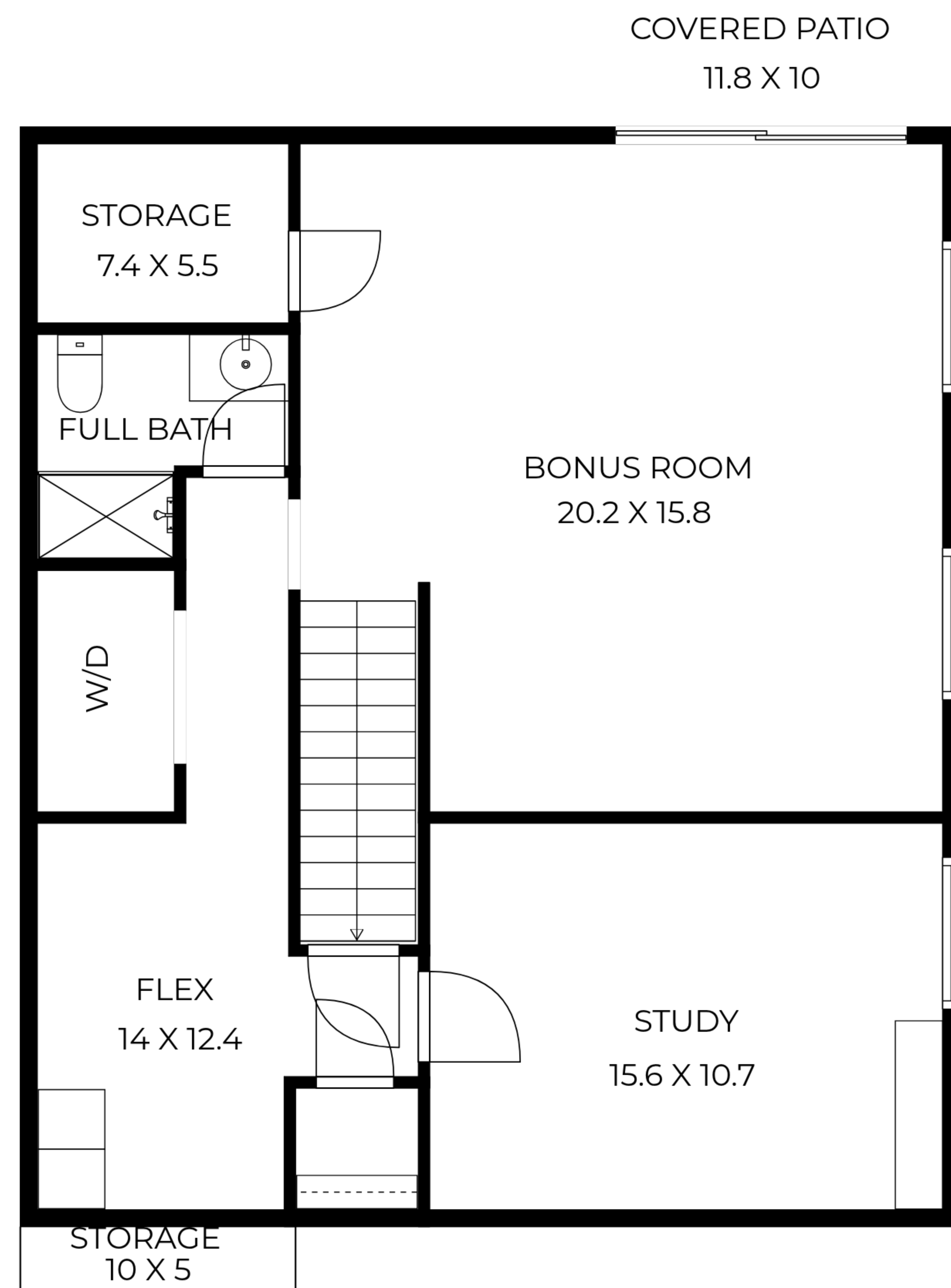
BASEMENT
