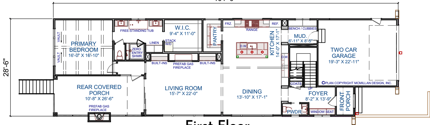
First Floor
