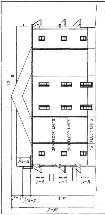
2521 FRIEDLAND PLACE BUILDING #15 TYPE B THREE STORY BUILDING FRONT ELEVATION SCALE - 3/32"=1'-0"
