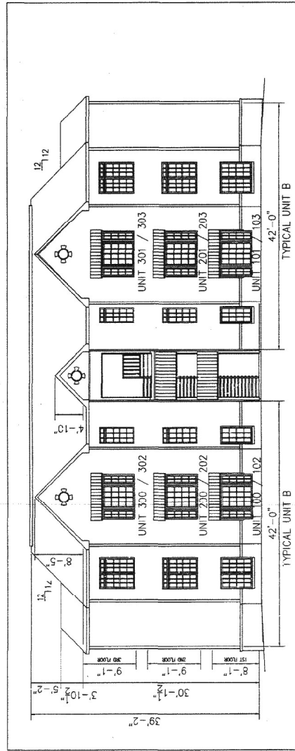
2521 FRIEDLAND PLACE BUILDING #15 TYPE B THREE STORY BUILDING FRONT ELEVATION SCALE - 3/32"=1'-0"
