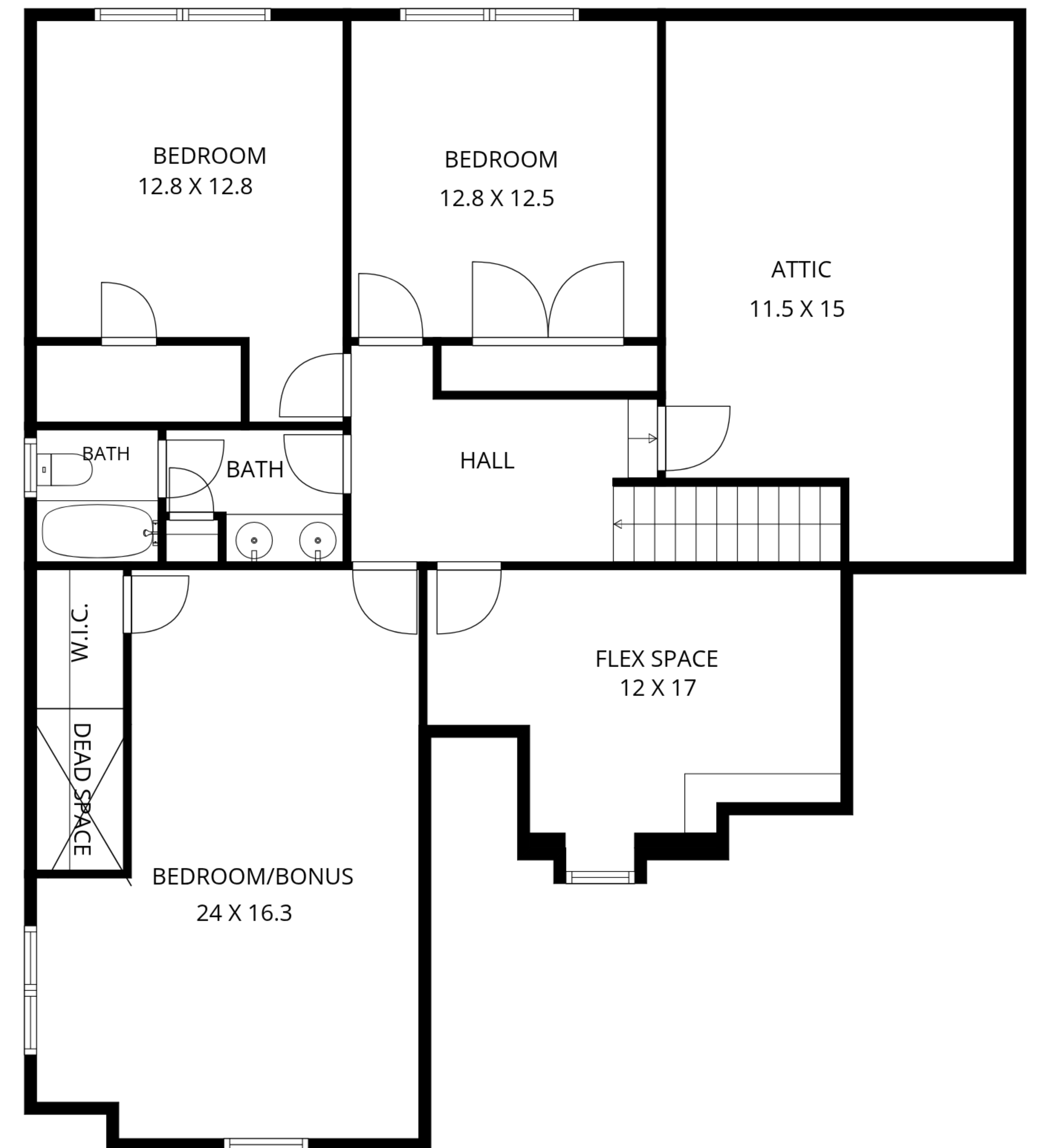
2ND FLOOR
