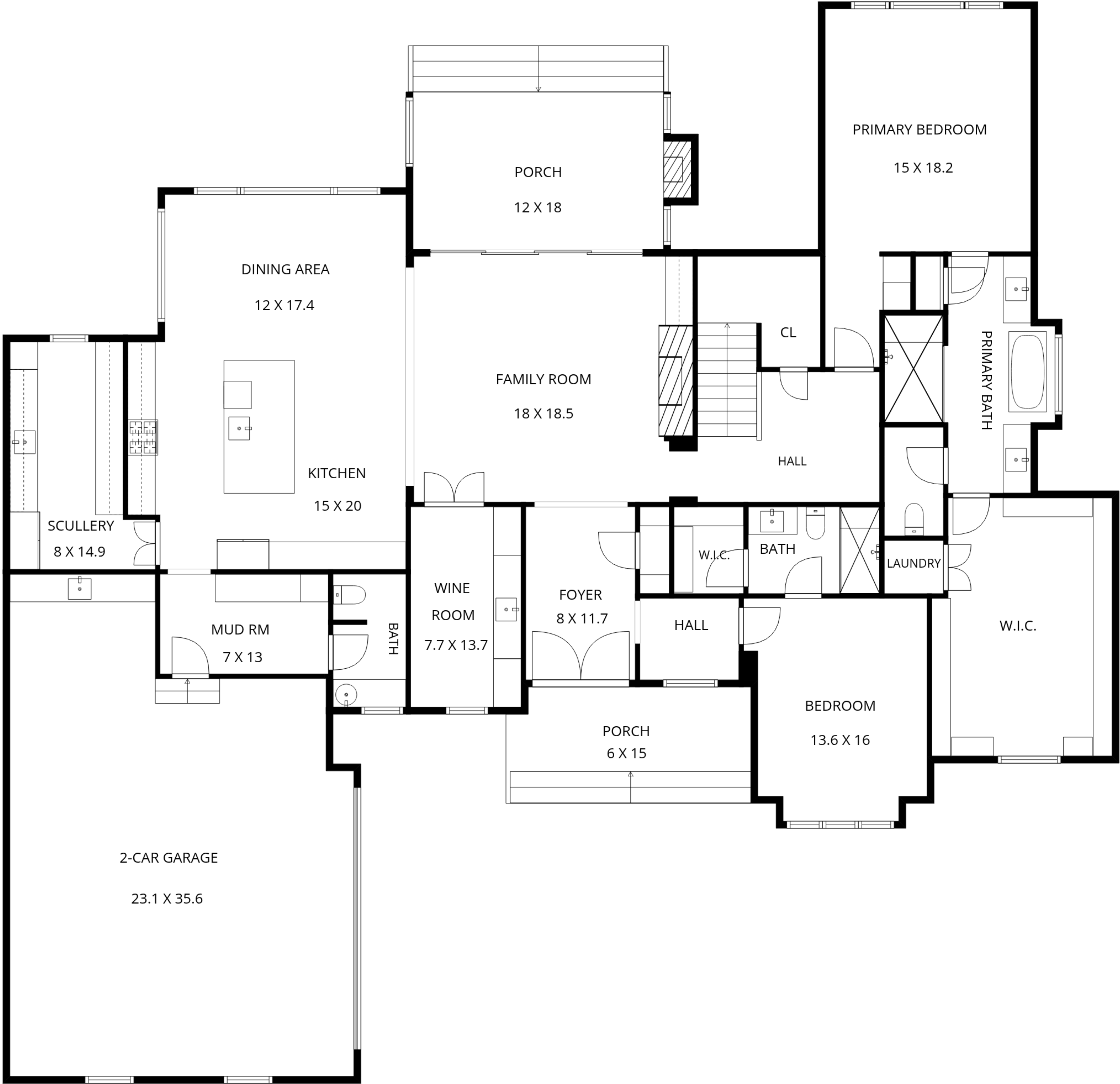
1ST FLOOR
