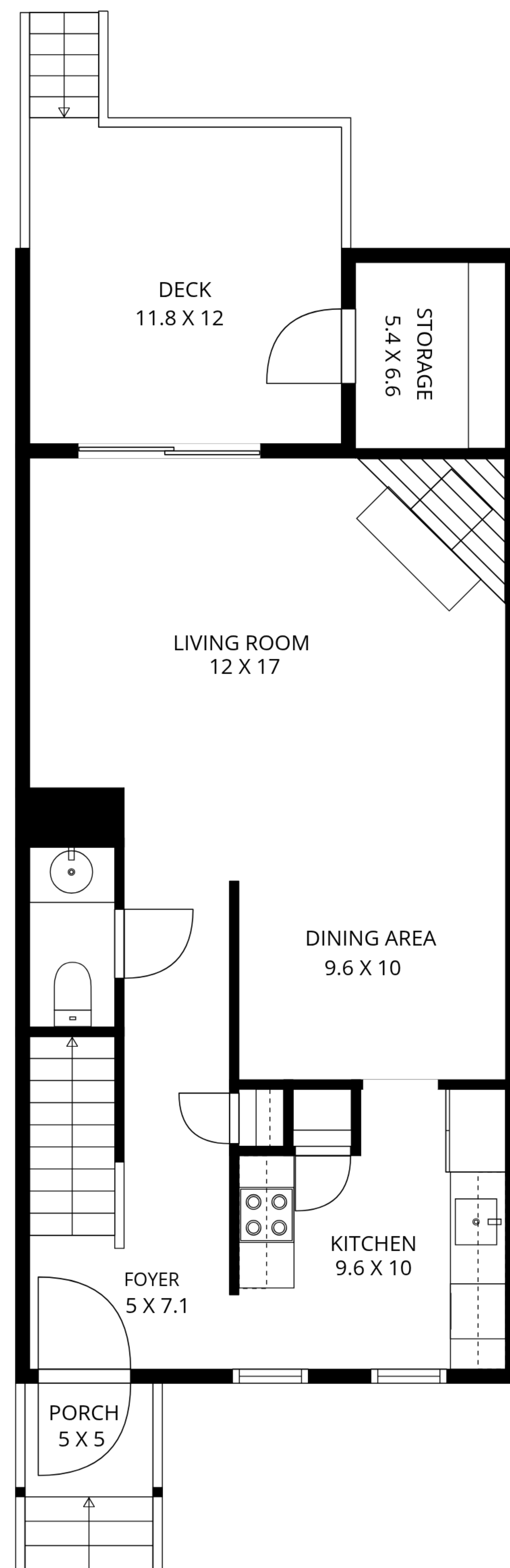
1ST FLOOR
