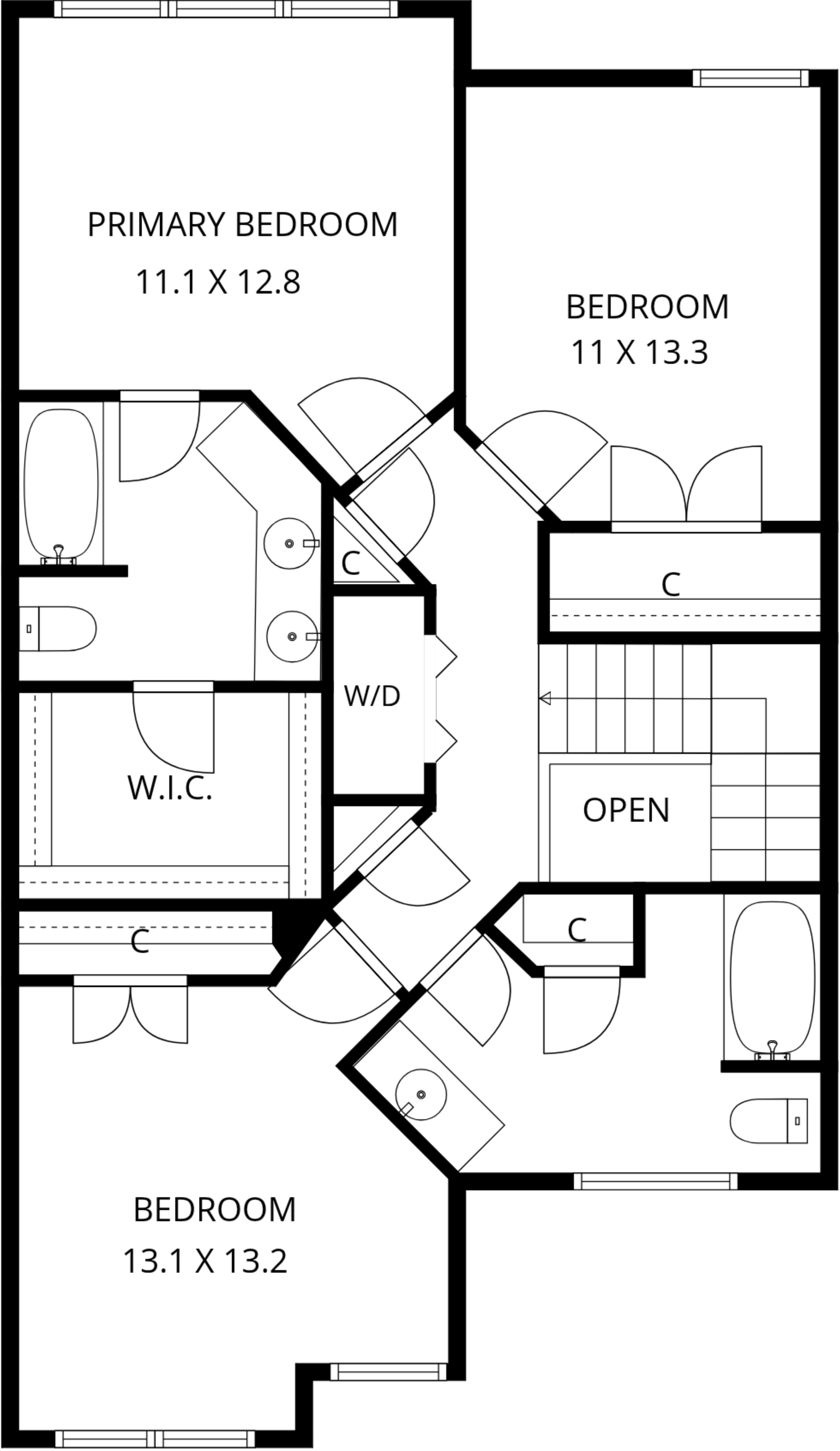
2ND FLOOR
