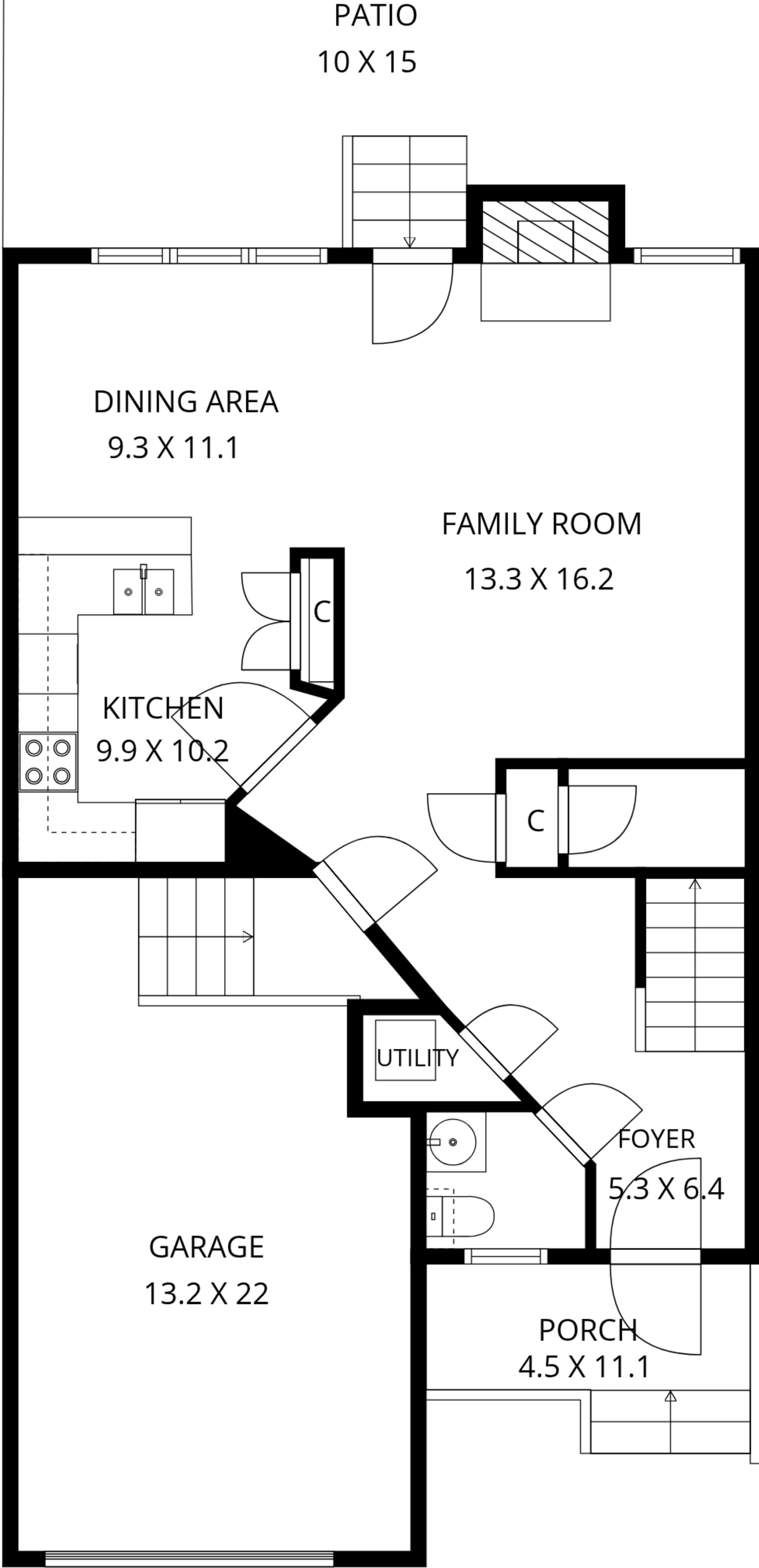
1ST FLOOR
