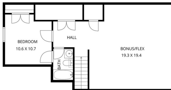
THIRD FLOOR
