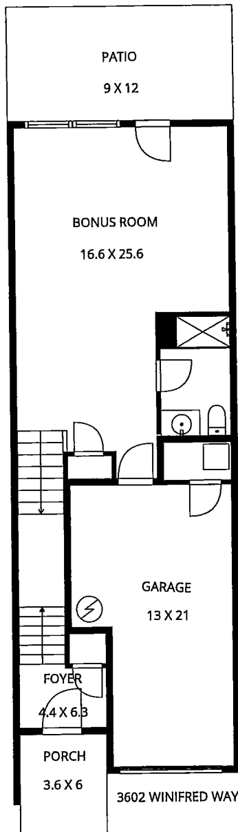
1ST FLOOR
