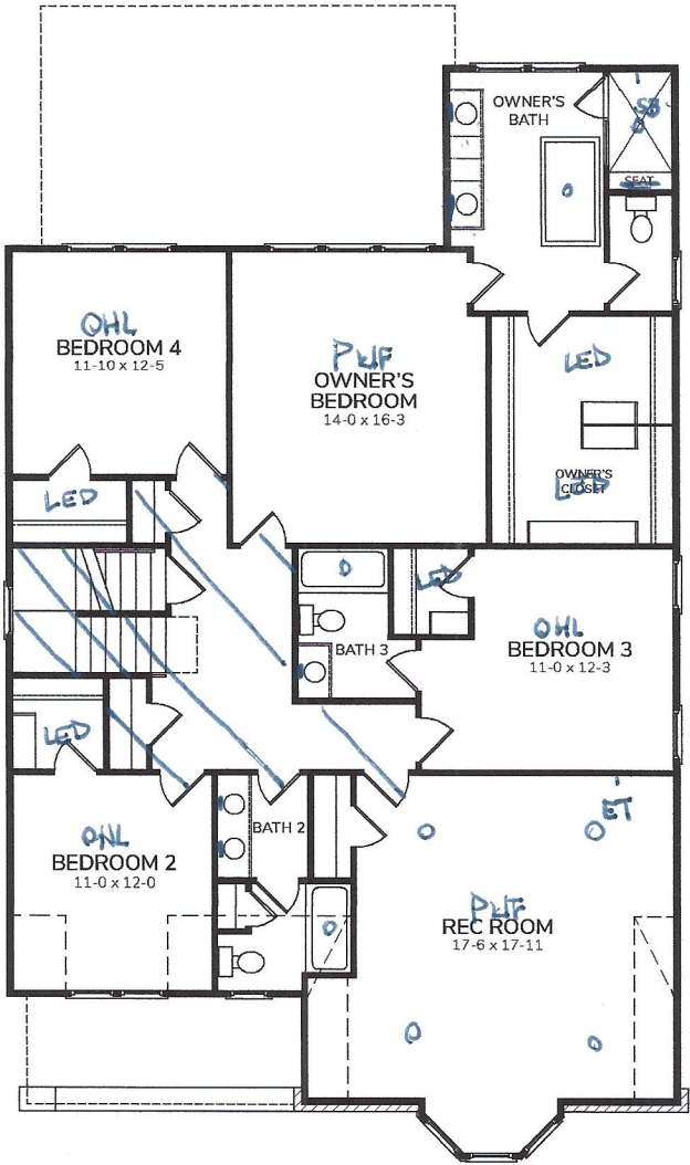
Second Floor
