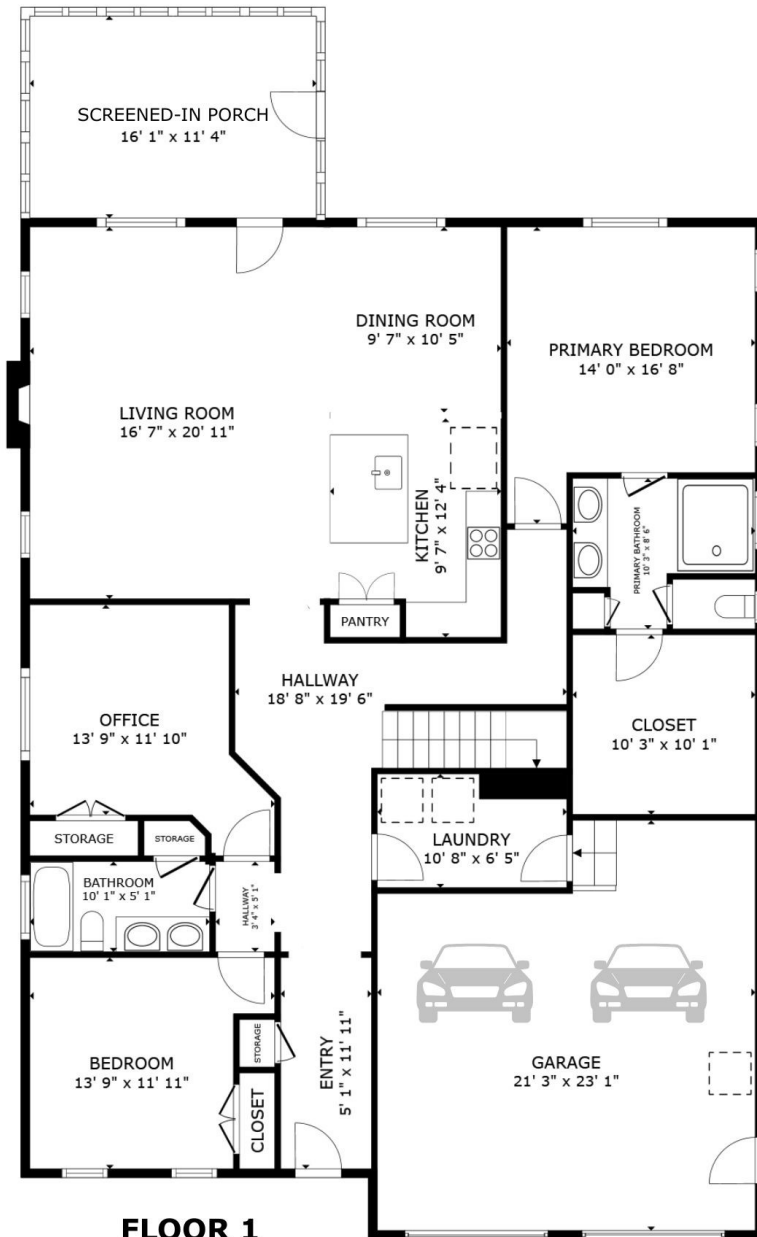
FLOOR 1 1,864 SQ.FT.
