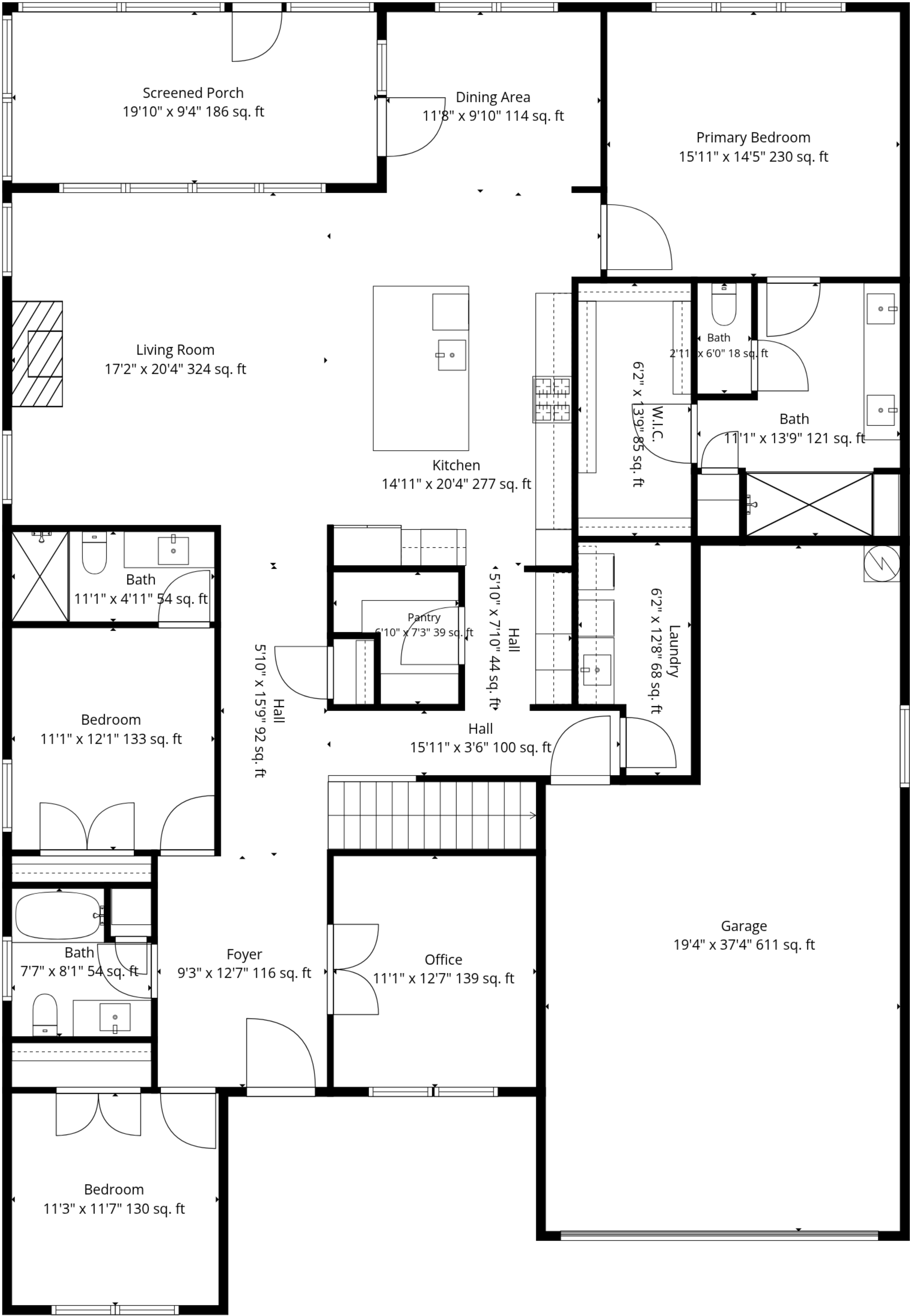
1st Floor
