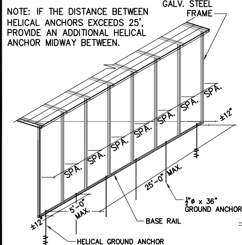
HELICAL GROUND ANCHORS
