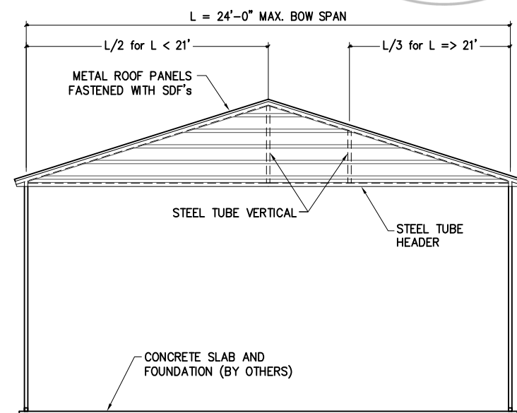
GABLE END ELEVATION
