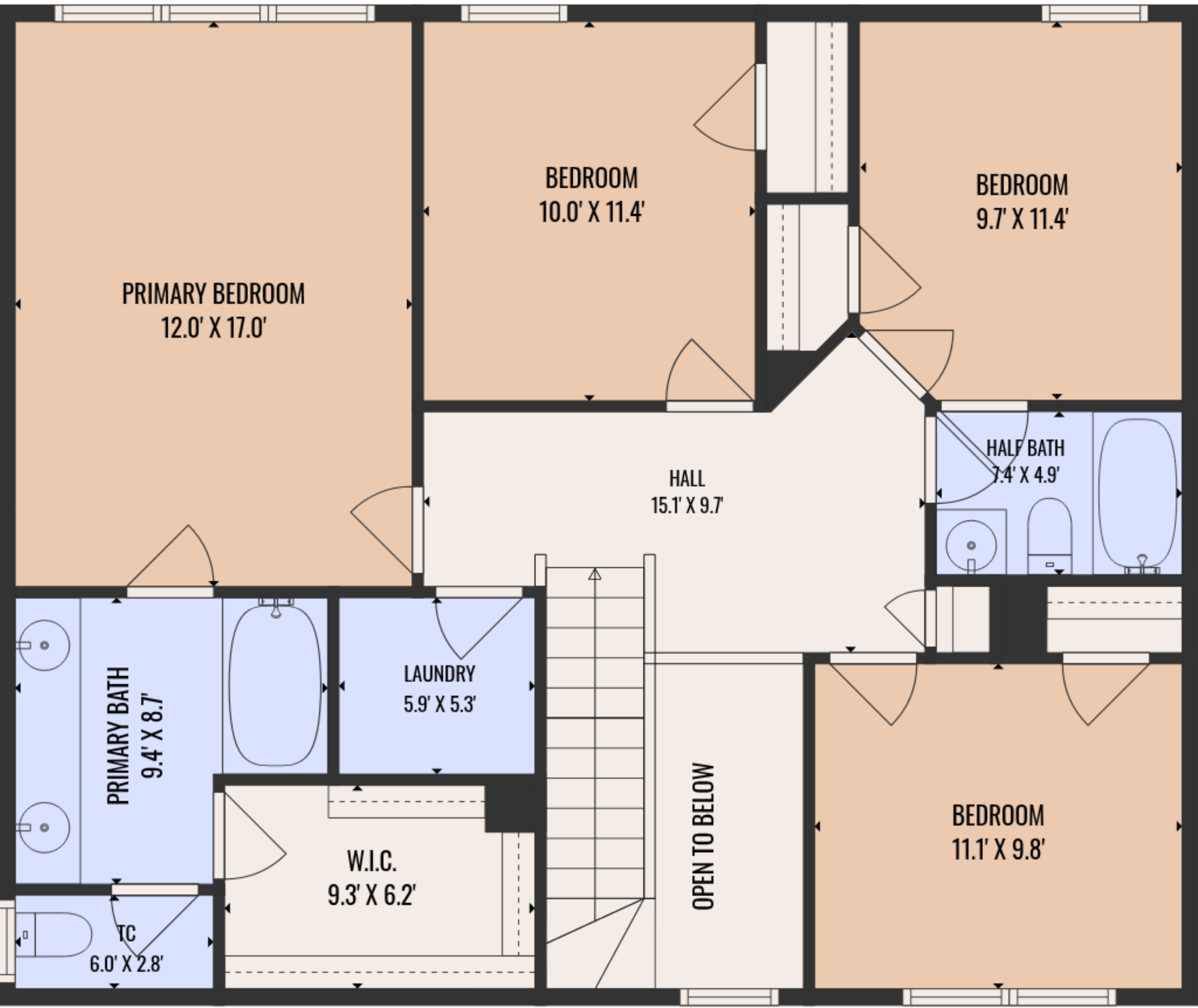
2ND FLOOR
