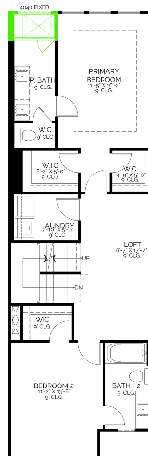
SECOND FLOOR
