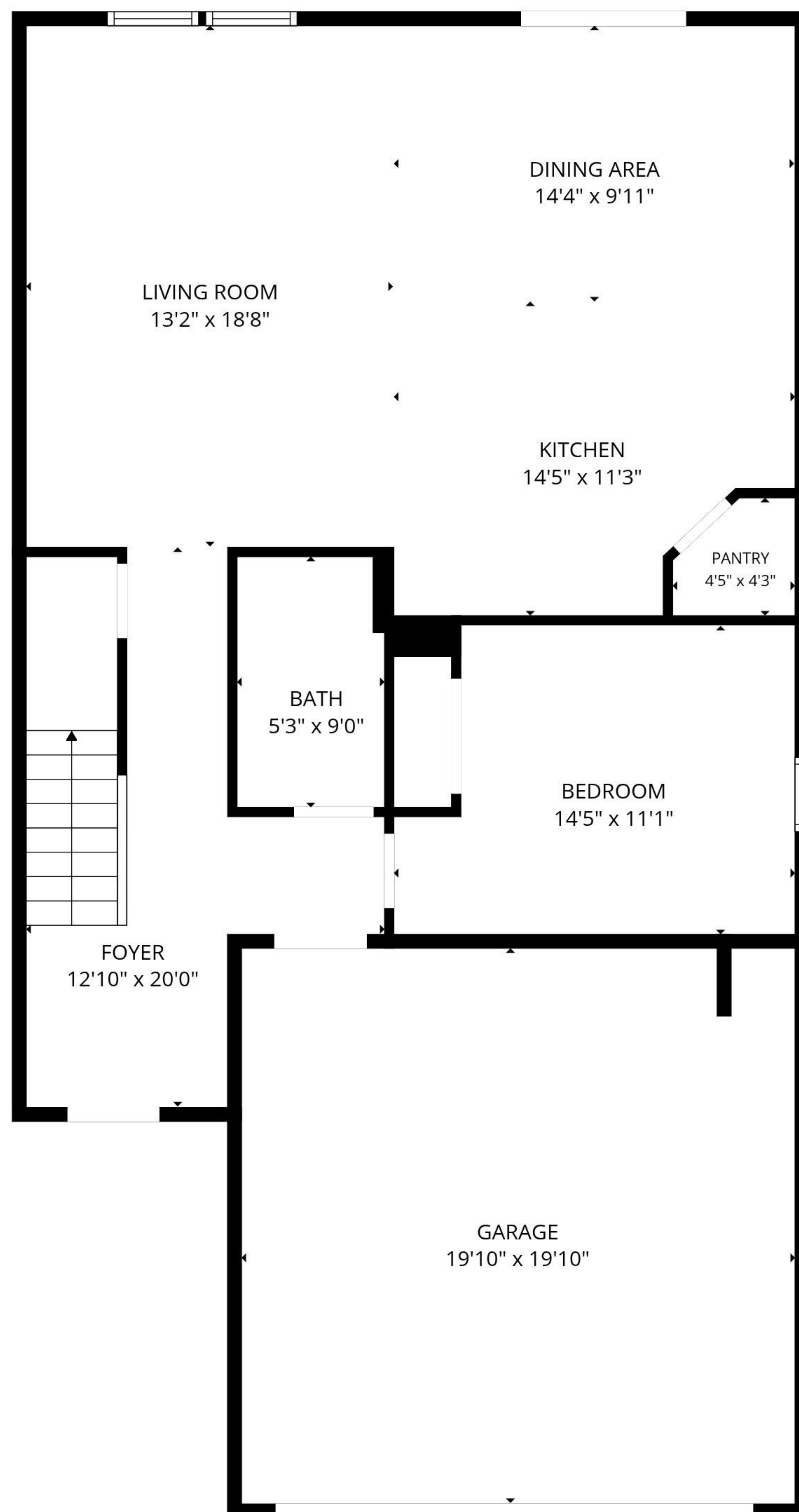
1st floor
