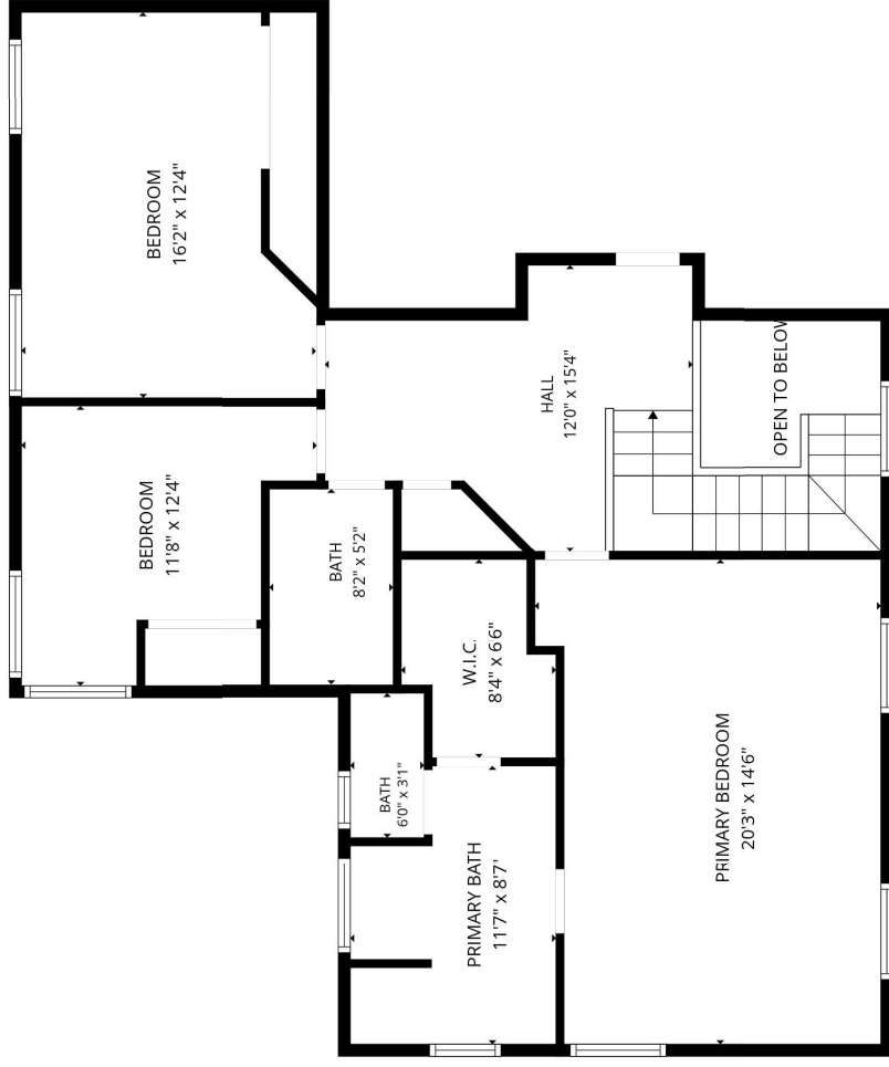
2nd floor
