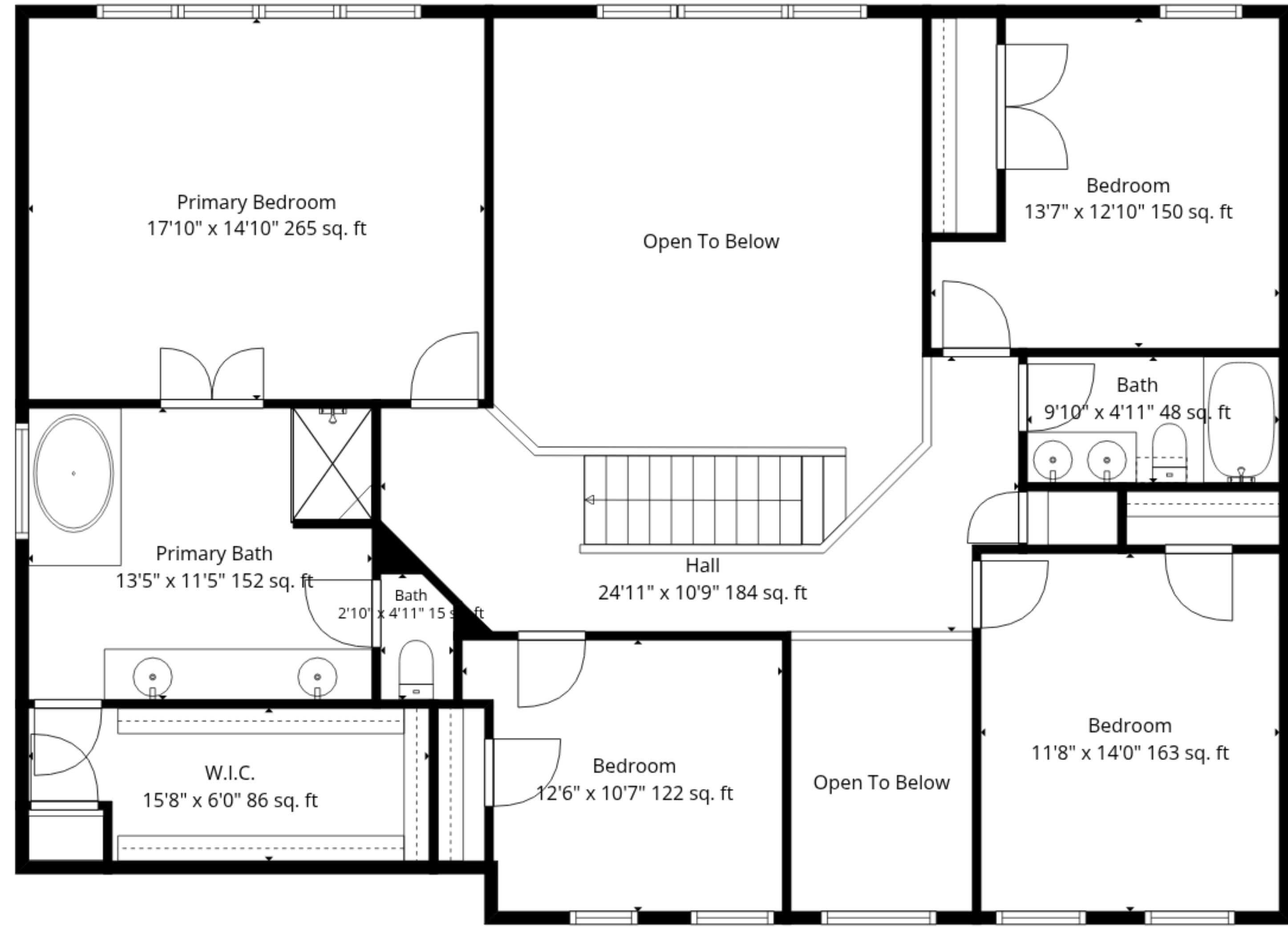
2nd Floor
