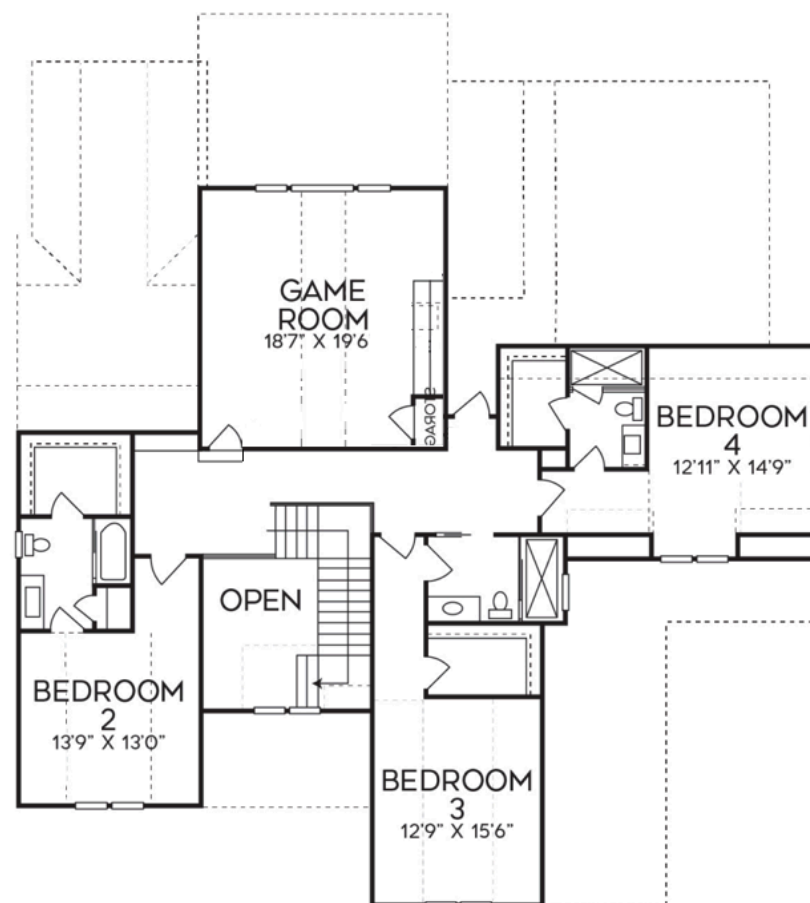
SECOND FLOOR
