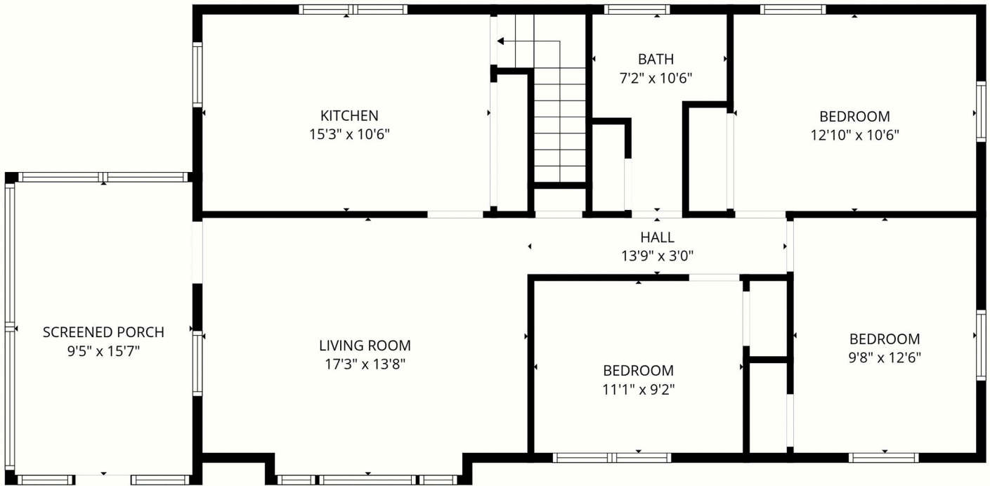
1st floor
