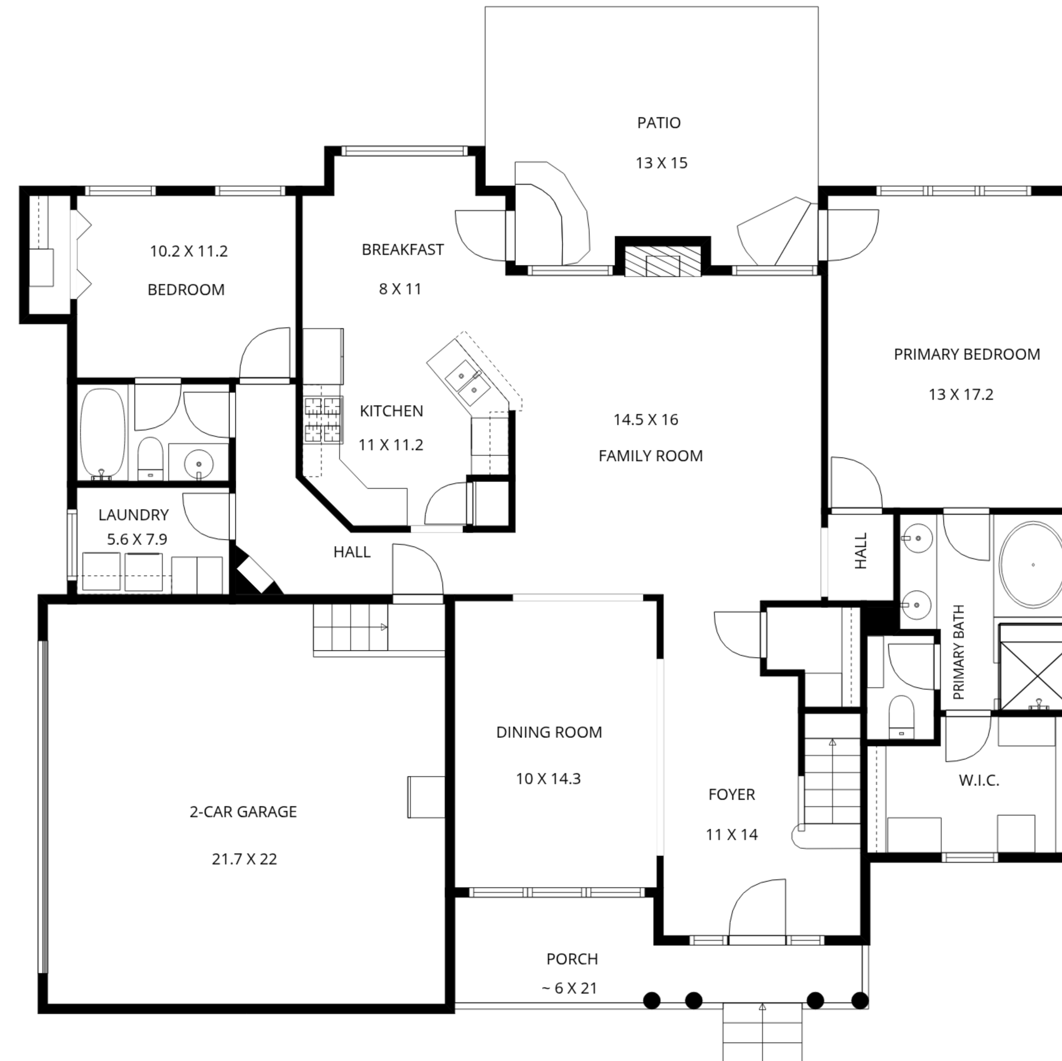
1ST FLOOR
