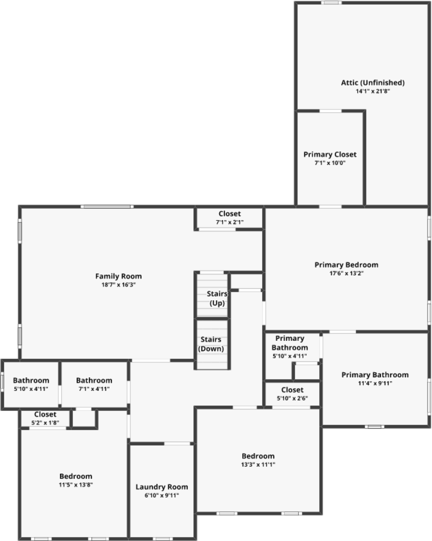
FLOOR 2
