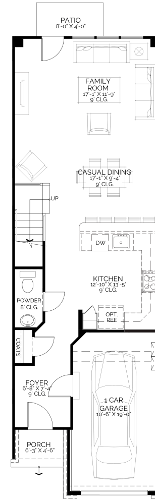
MAIN FLOOR
