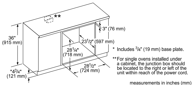
Dimensions for Under-Counter Installation
