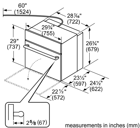
Single Oven Bottom Hinge
