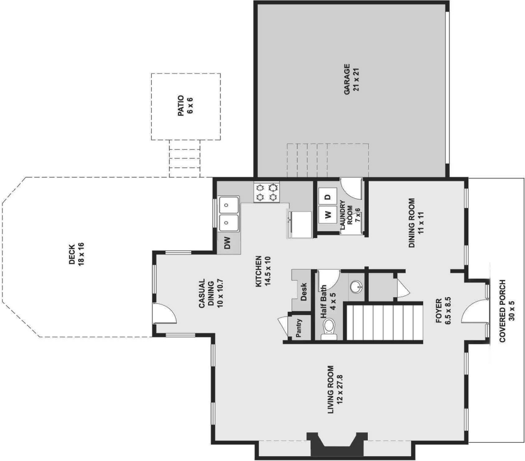
FIRST FLOOR
