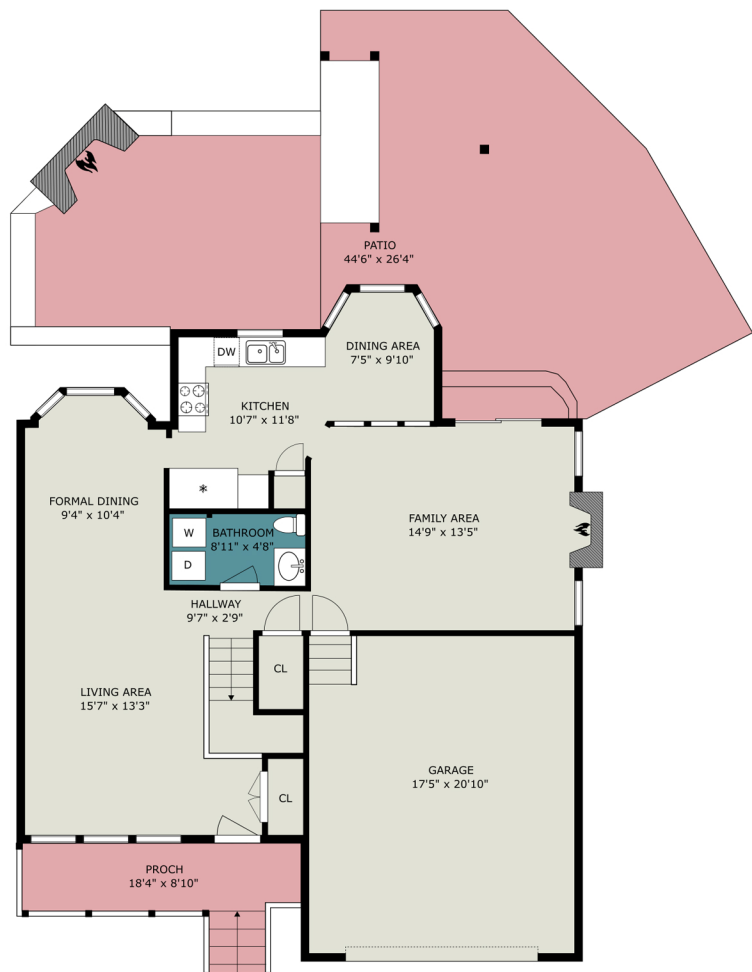
First Floor
