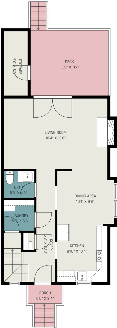
First Floor
