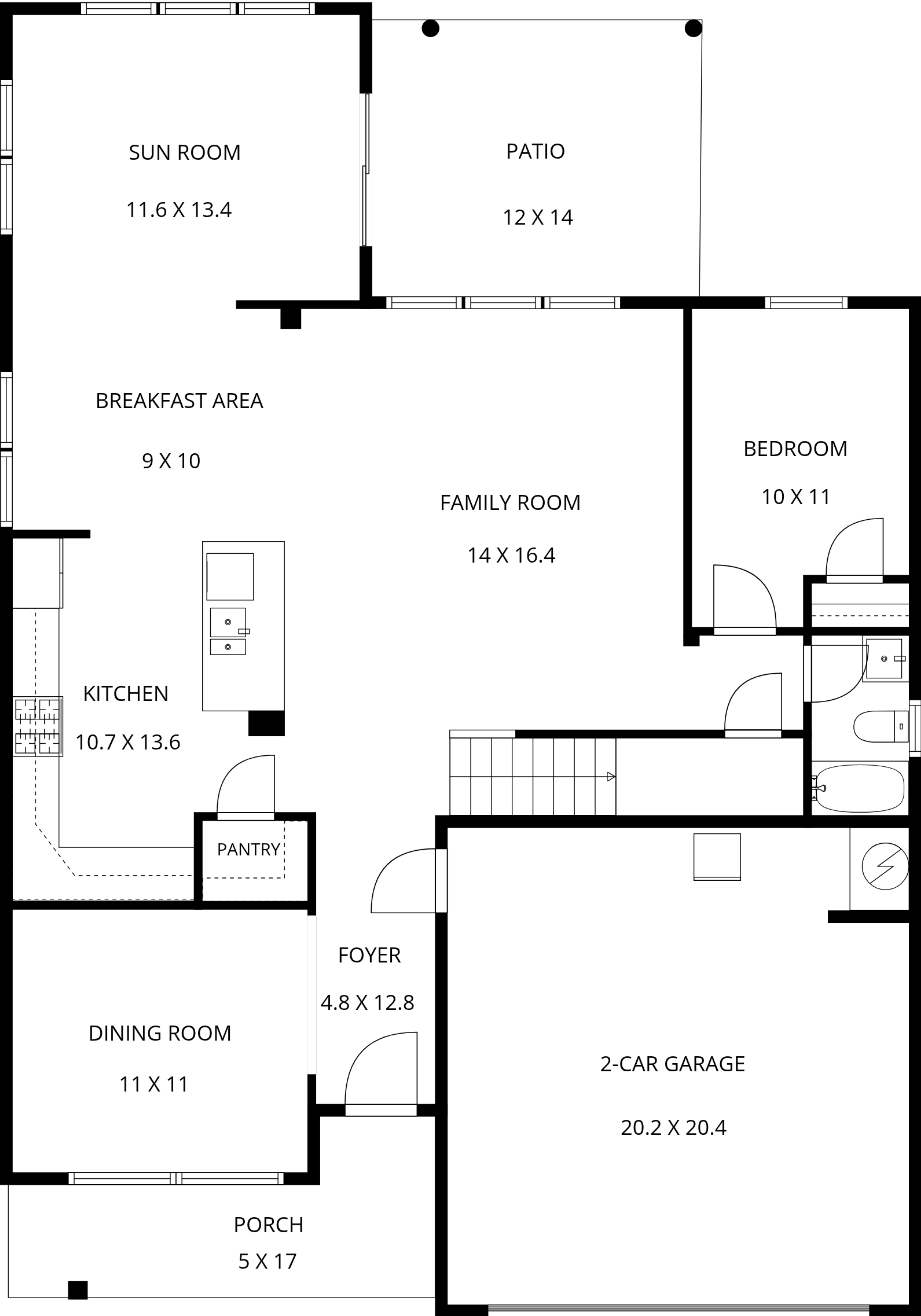
1ST FLOOR
