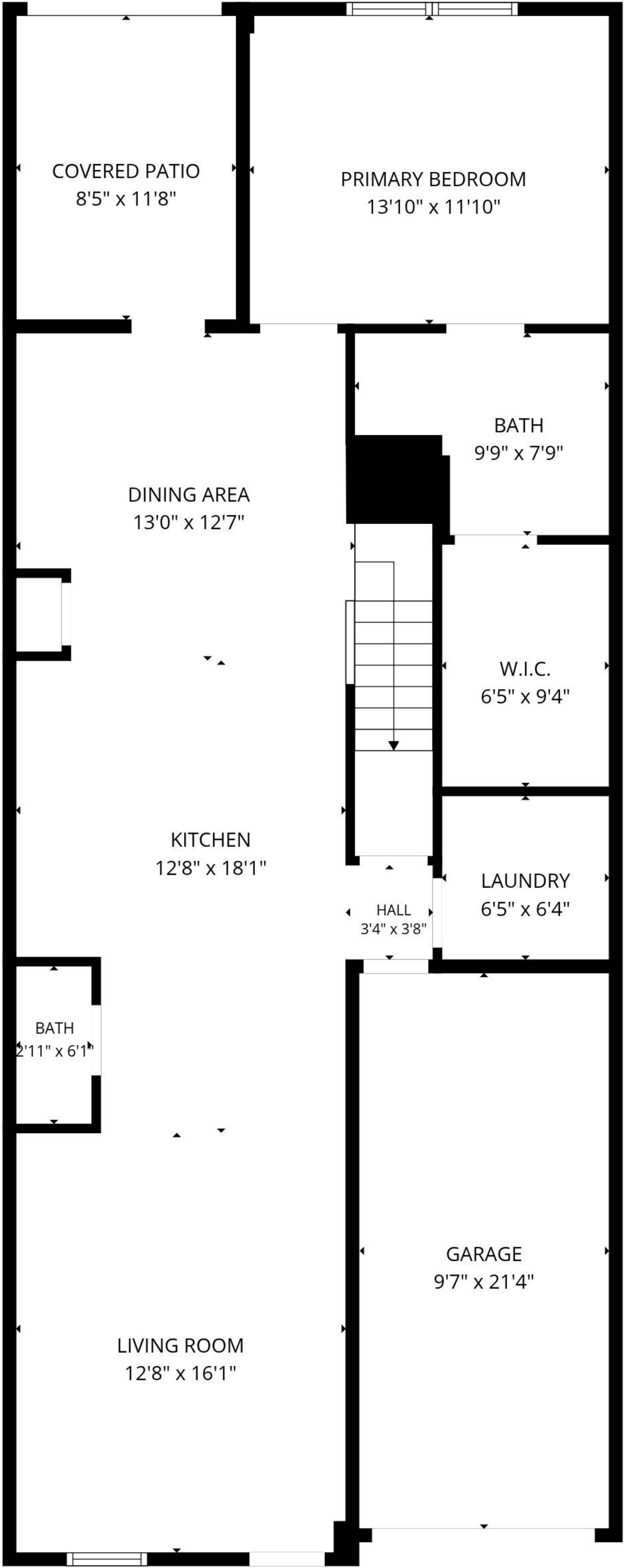
1st floor
