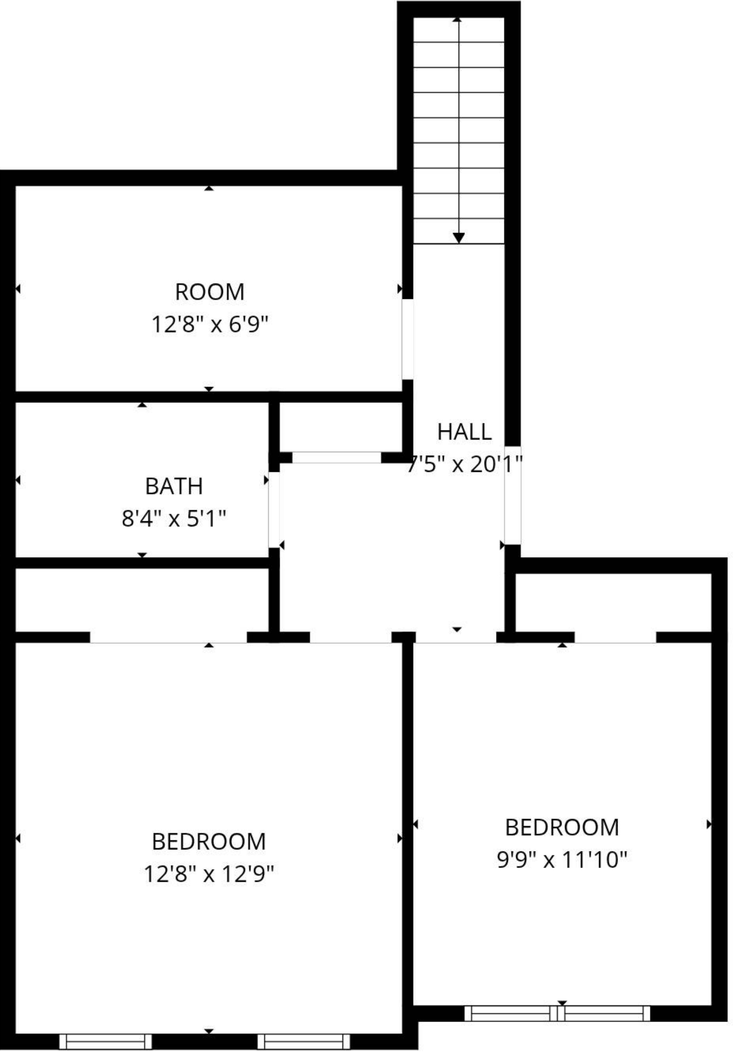
2nd floor
