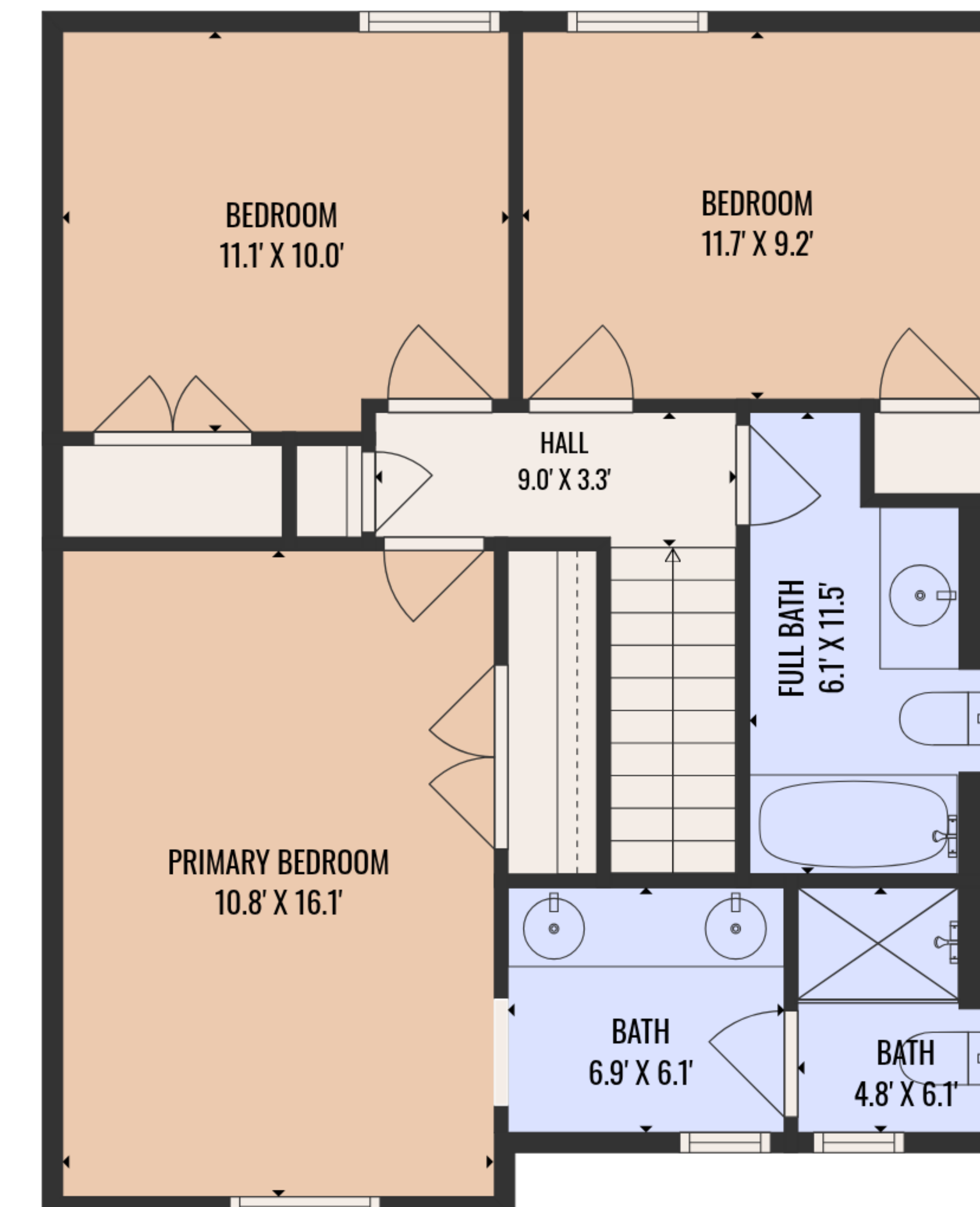
2ND FLOOR
